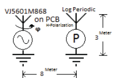
Fig. 3 - VJ5601M868 PCB Mounting and Coordinate Directions
