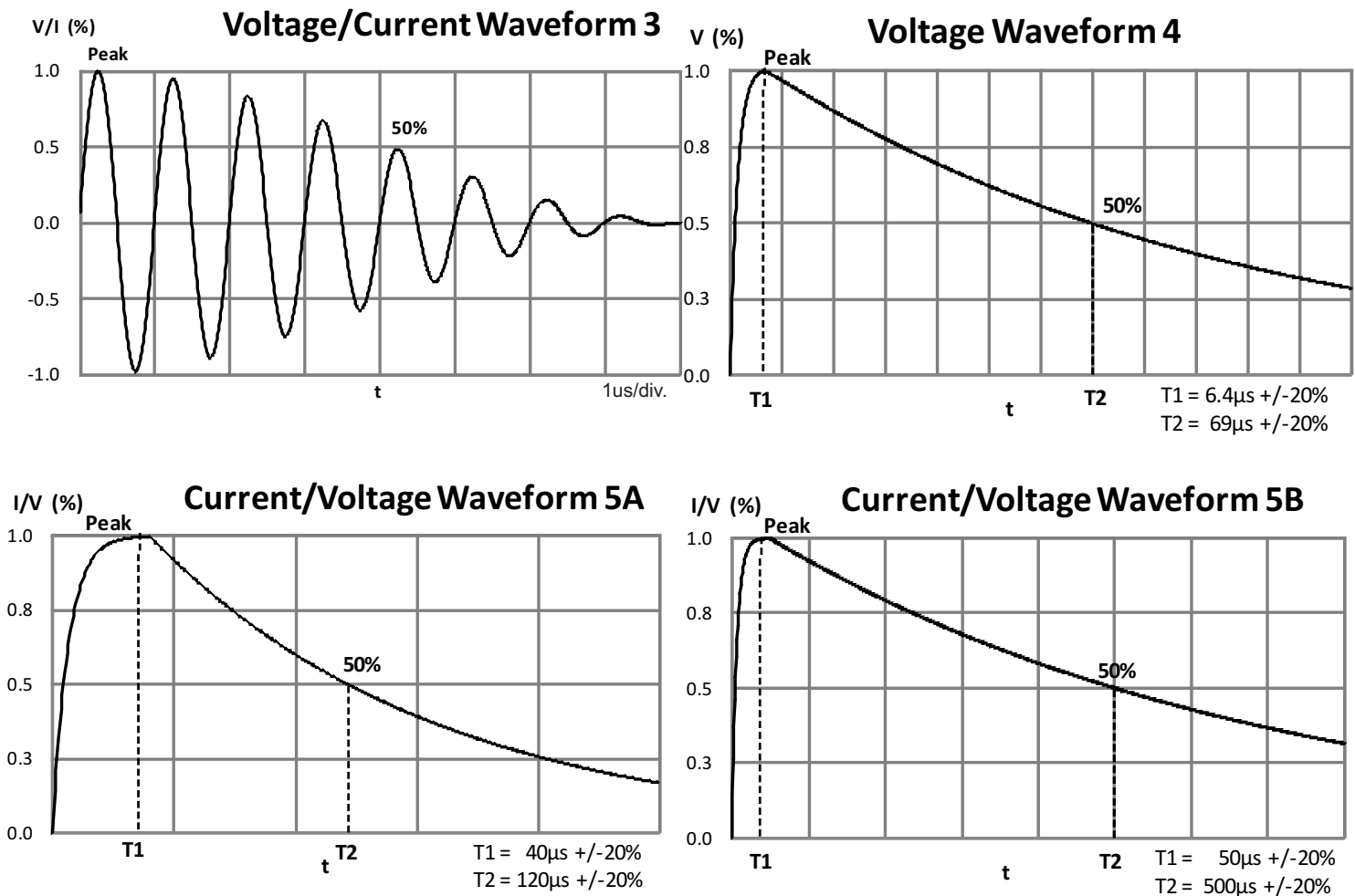
Figure 8. Lightning Waveforms
