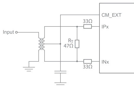
Figure 4. Transformer-Coupled Input
