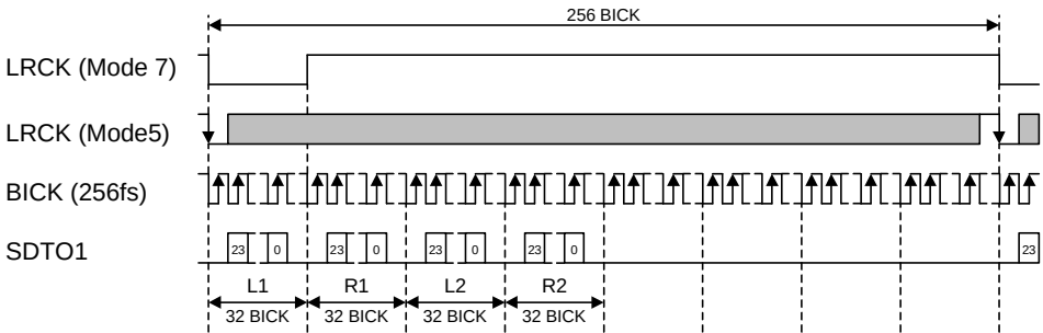
Figure 4. Mode 5, 7 Timing (TDM256 mode, I 2 S Compatible)
