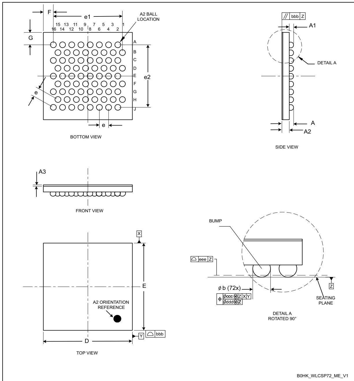
Figure 84. WLCSP72 - Outline
