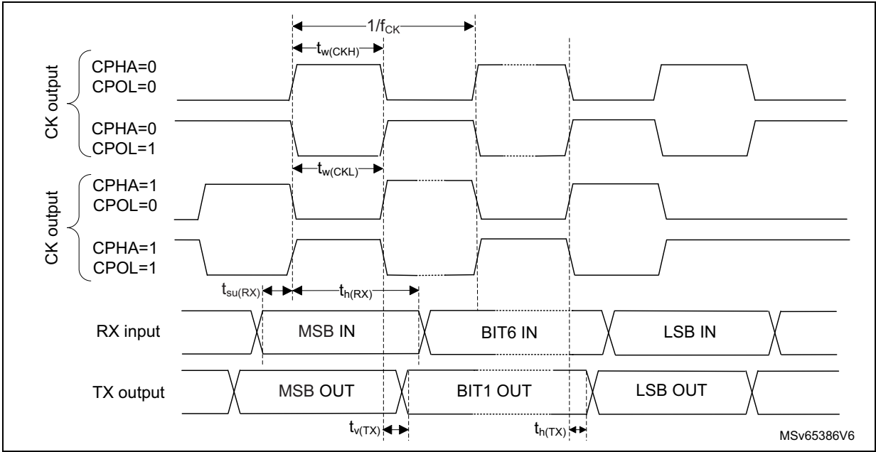
Figure 60. USART timing diagram in SPI master mode
