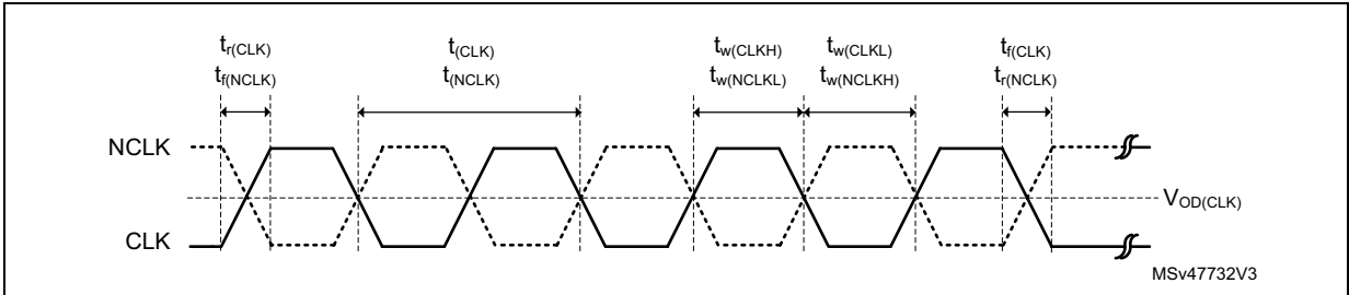
Figure 53. OCTOSPI HyperBus clock
