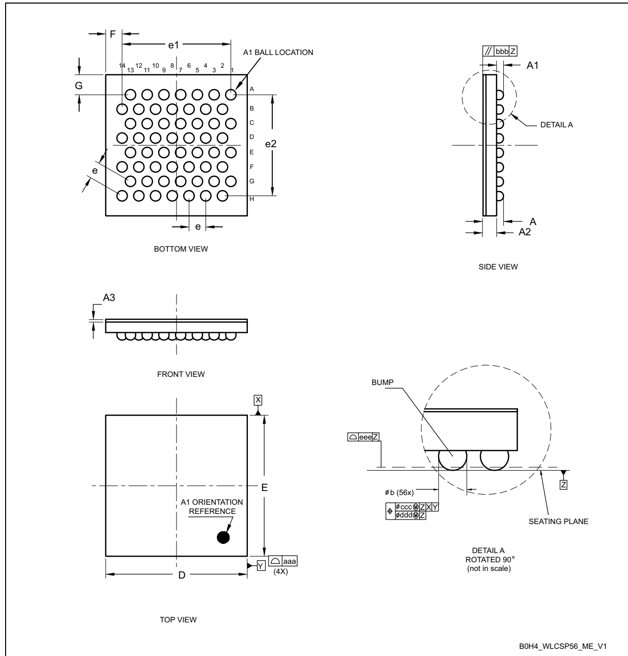
Figure 75. WLCSP56 - Outline
