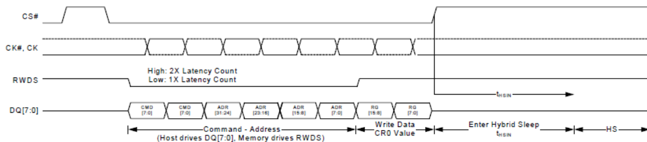
Figure 6.2 Enter HS transaction
