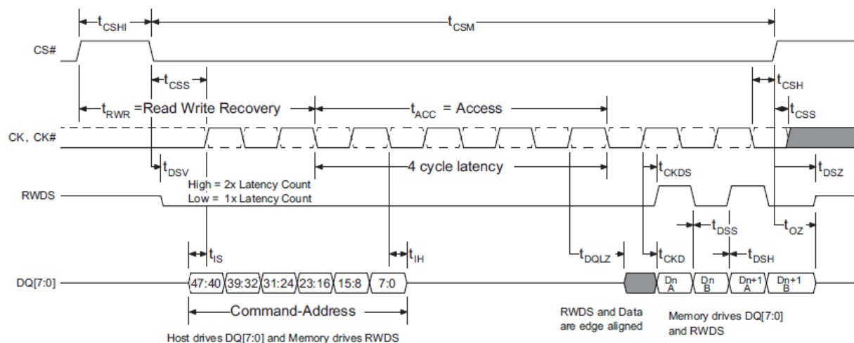
Figure 10.6 Read Timing Diagram — With Additional Latency Required
