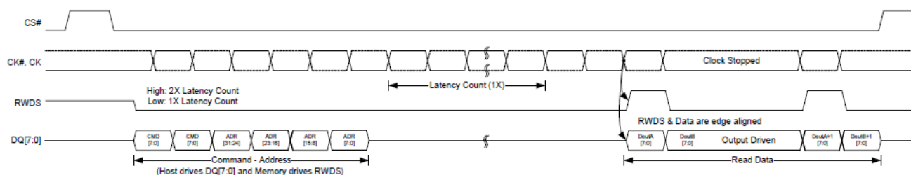
Figure 6.1 Active clock stop during read transaction (DDR)
