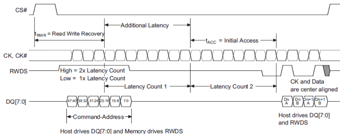
Figure 3.5 Write Transaction with additional initial latency
