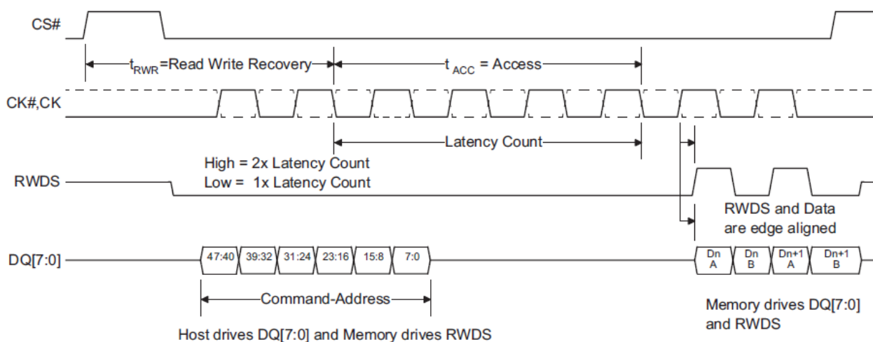
Figure 1.1 Read Transaction, Single Initial Latency Count
