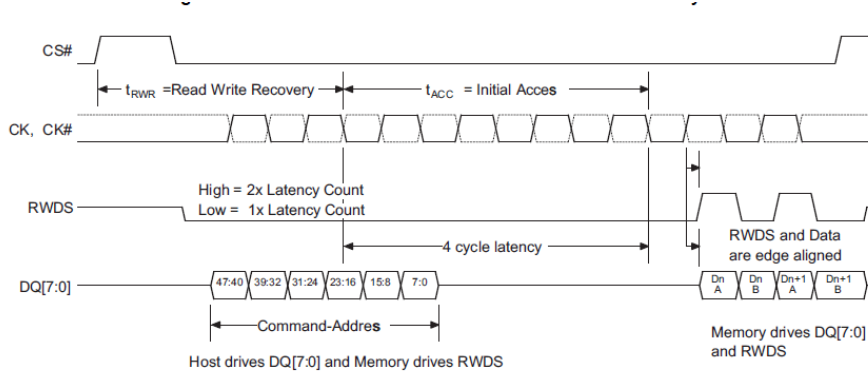
Figure 3.5 Read Transaction without additional initial latency
