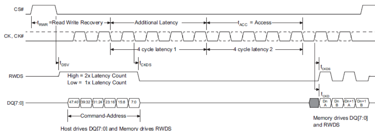
Figure 10.7 Read Timing Diagram — Data valid timing
