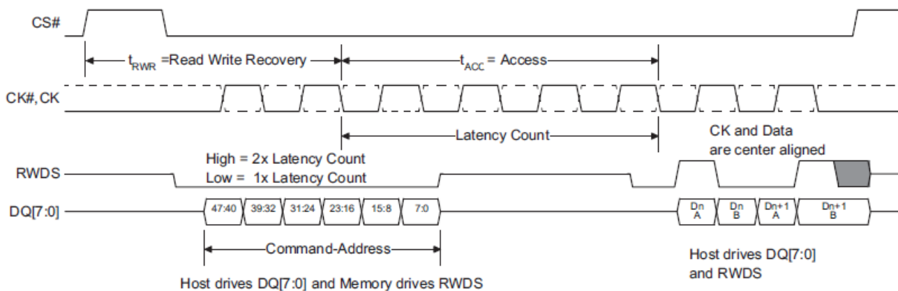
Figure 1.3 Write Transaction, Single Initial Latency Count
