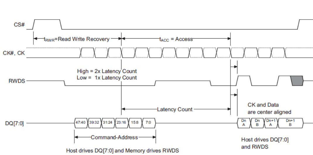
Figure 3.5 Write Transaction without additional initial latency
