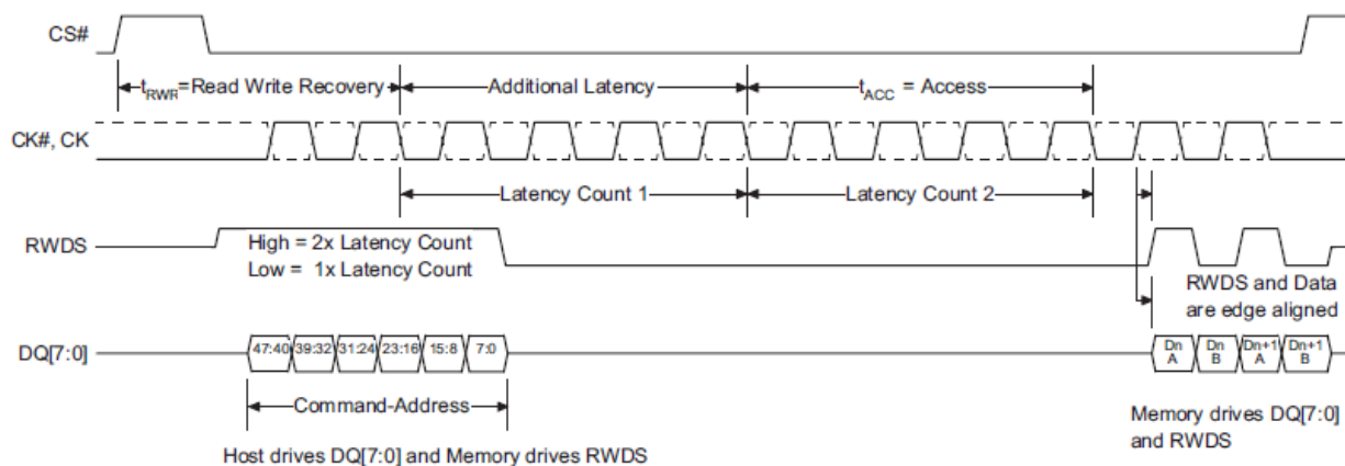
Figure 1.2 Read Transaction, Additional Latency Count
