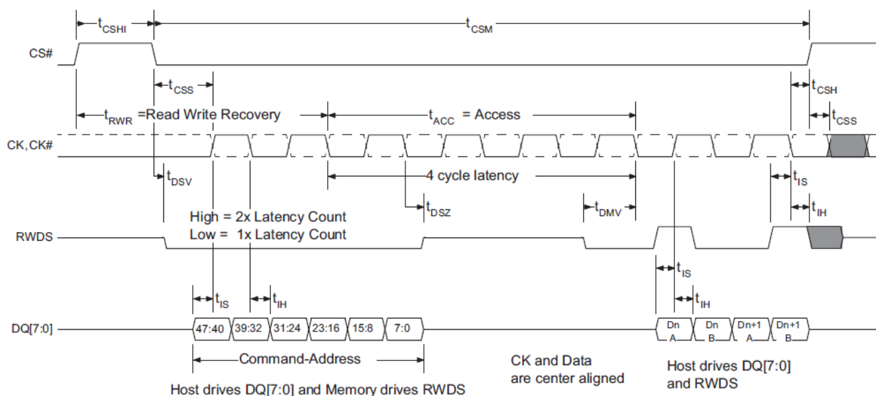
Figure 10.8 Write Timing Diagram — No Additional Latency
