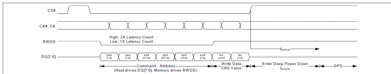
Figure 6.4 Enter DPD transaction
