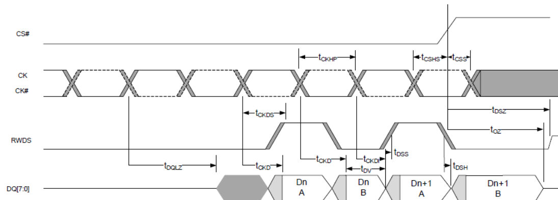
Figure 10.7 Read Timing Diagram — Data valid timing
