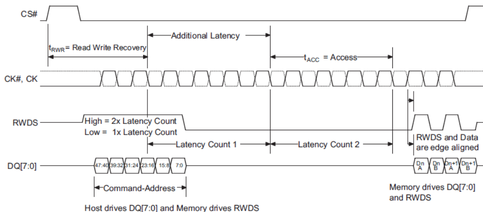
Figure 3.4 Read Transaction with additional initial latency
