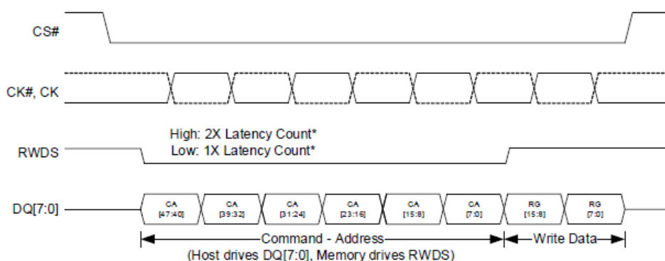
Figure 3.6 Write Transaction without additional initial latency
