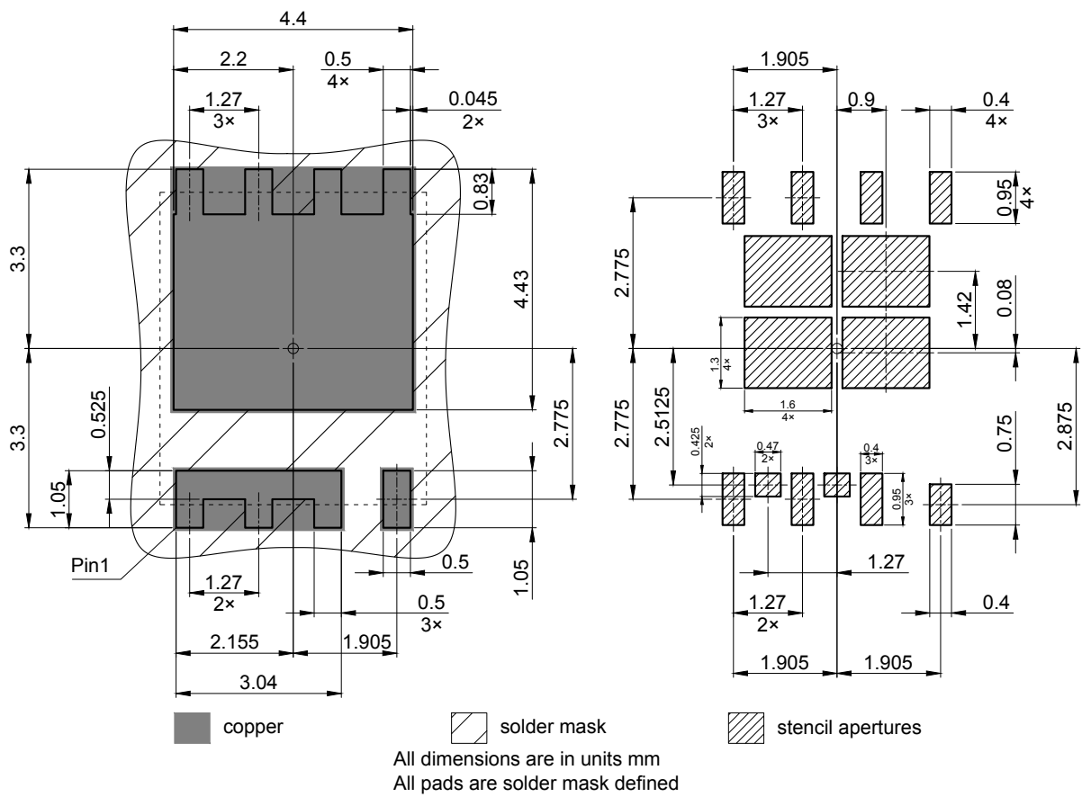
Figure 3 Bonding diagram PG-VSON-8 / PG-WSON-8, dimensions in mm
