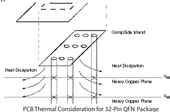
PCB Thermal Consideration for 32-Pin QFN Package
