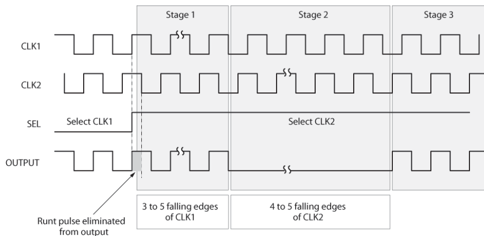
Figure 2. Timing Diagram 1
