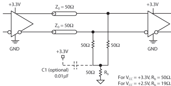
Figure 4b. Parallel Termination (3-Resistors)
