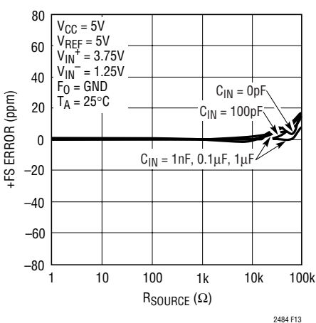
Figure 13. +FS Error vs R_{SQUBCE} at IN^+ or IN^-
