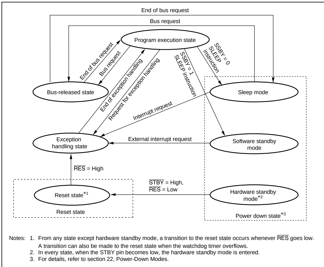
Figure 2.13 State Transitions
