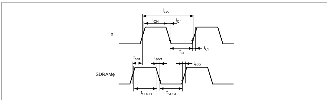
Figure 24.3 SDRAMφ Timing*
