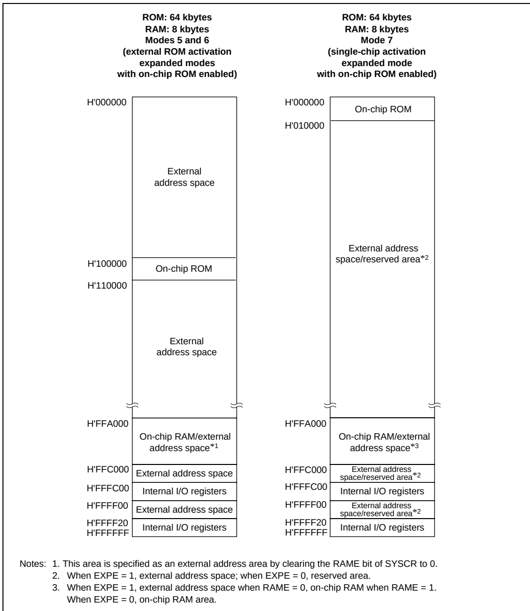
Figure 3.3 H8S/2673 Memory Map (2)
