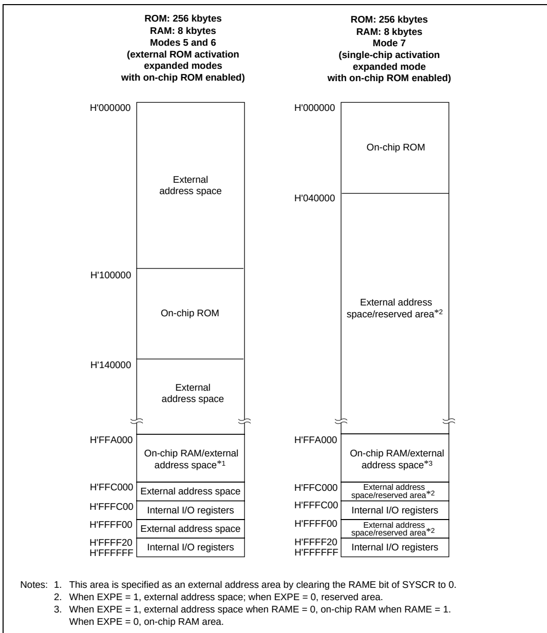
Figure 3.1 H8S/2676 Memory Map (2)
