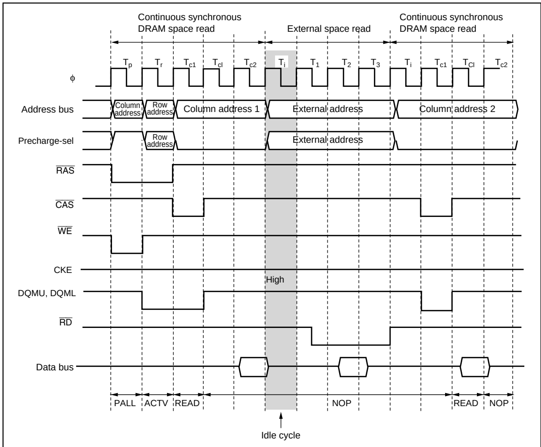
Figure 6.79 Example of Idle Cycle Operation after Continuous Synchronous DRAM Space Read Access (Read between Different Area) (IDL = 0, CAS Latency 2)
