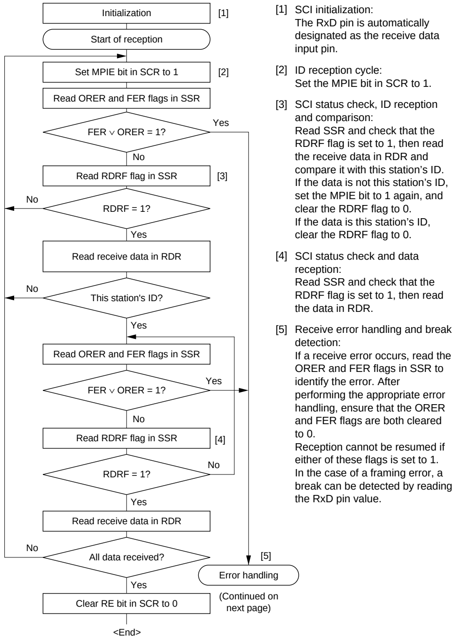
Figure 15.13 Sample Multiprocessor Serial Reception Flowchart (1)
