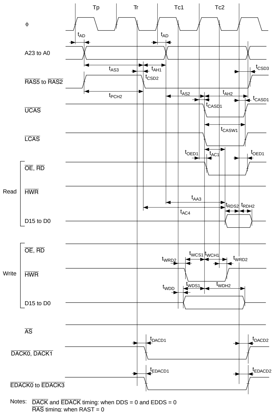
Figure 24.14 DRAM Access Timing: Two-State Access
