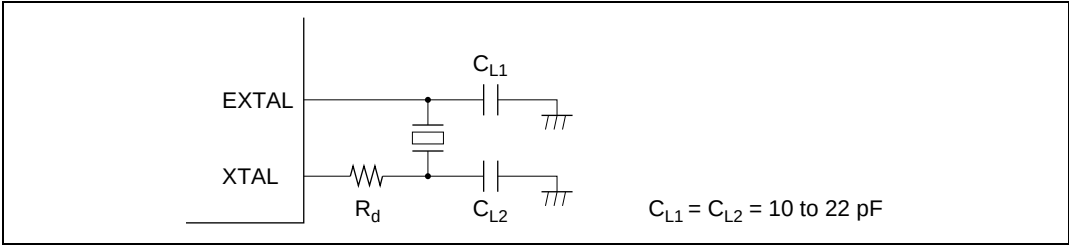
Figure 21.2 Connection of Crystal Resonator (Example)
