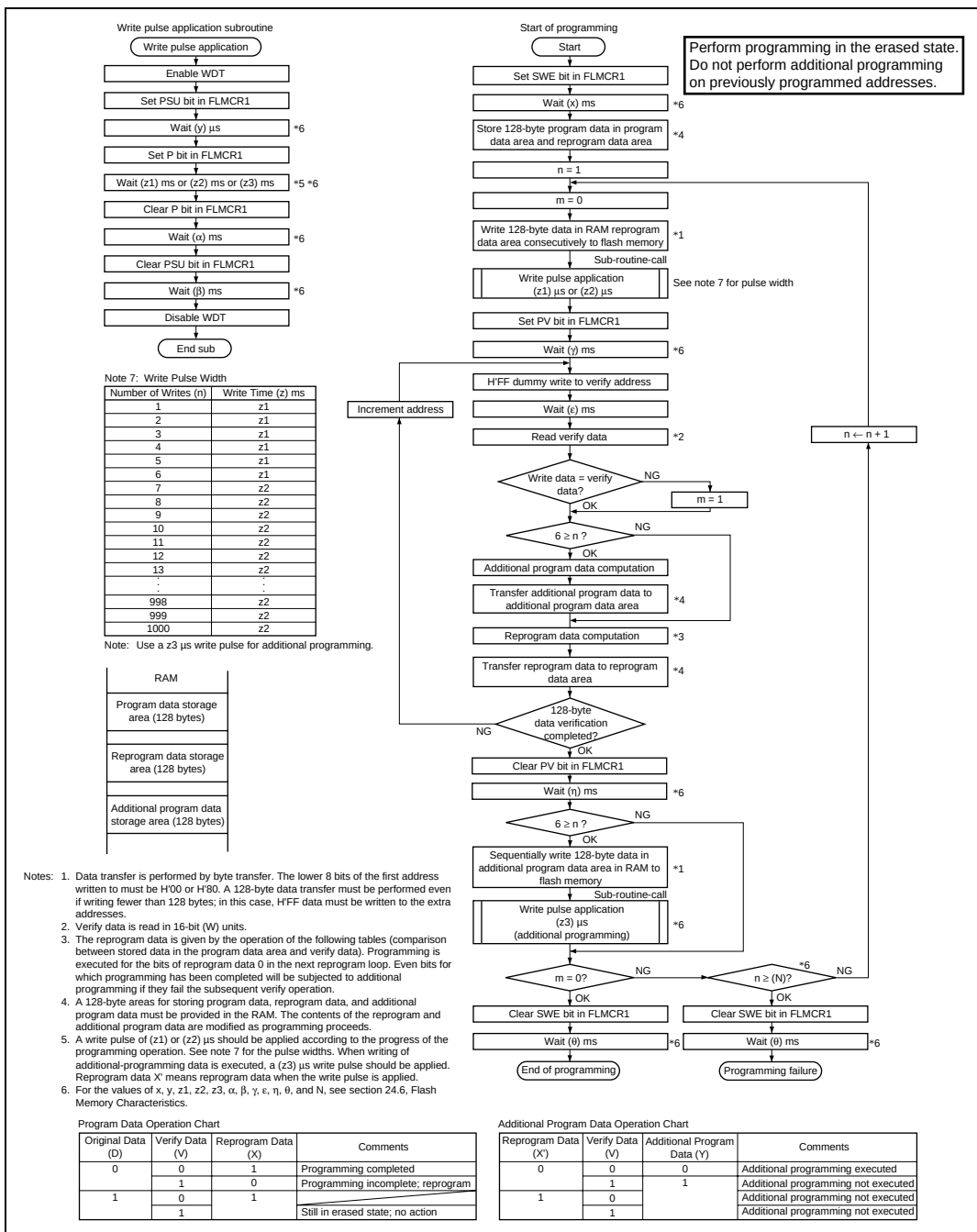
Figure 19.10 Program/Program-Verify Flowchart
