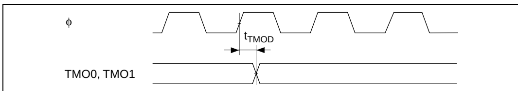
Figure 24.38 8-Bit Timer Output Timing
