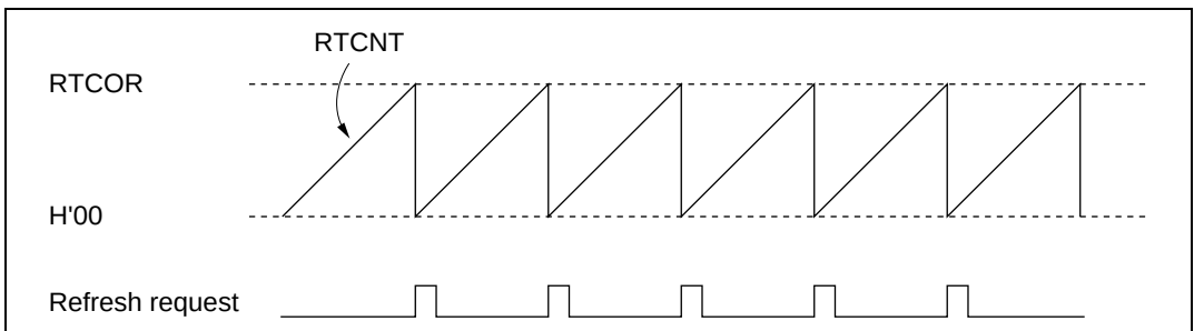
Figure 6.34 RTCNT Operation
