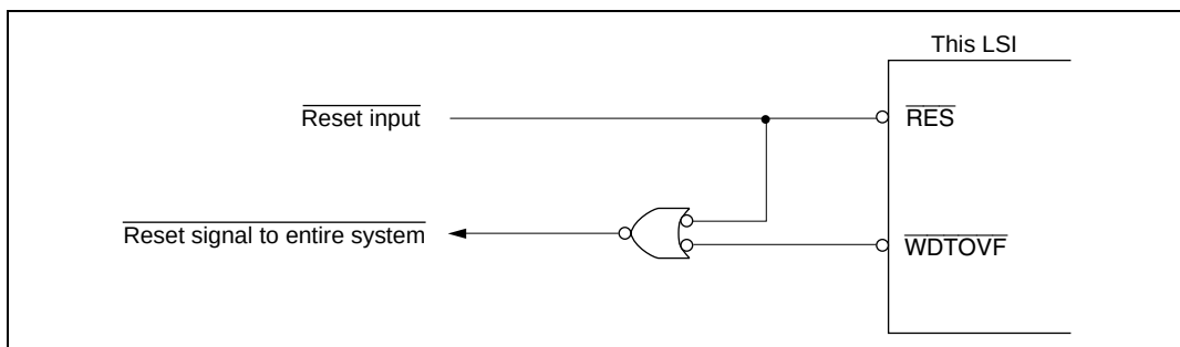
Figure 14.6 Circuit for System Reset by \overline{\text{WDTOVF}} Signal (Example)
