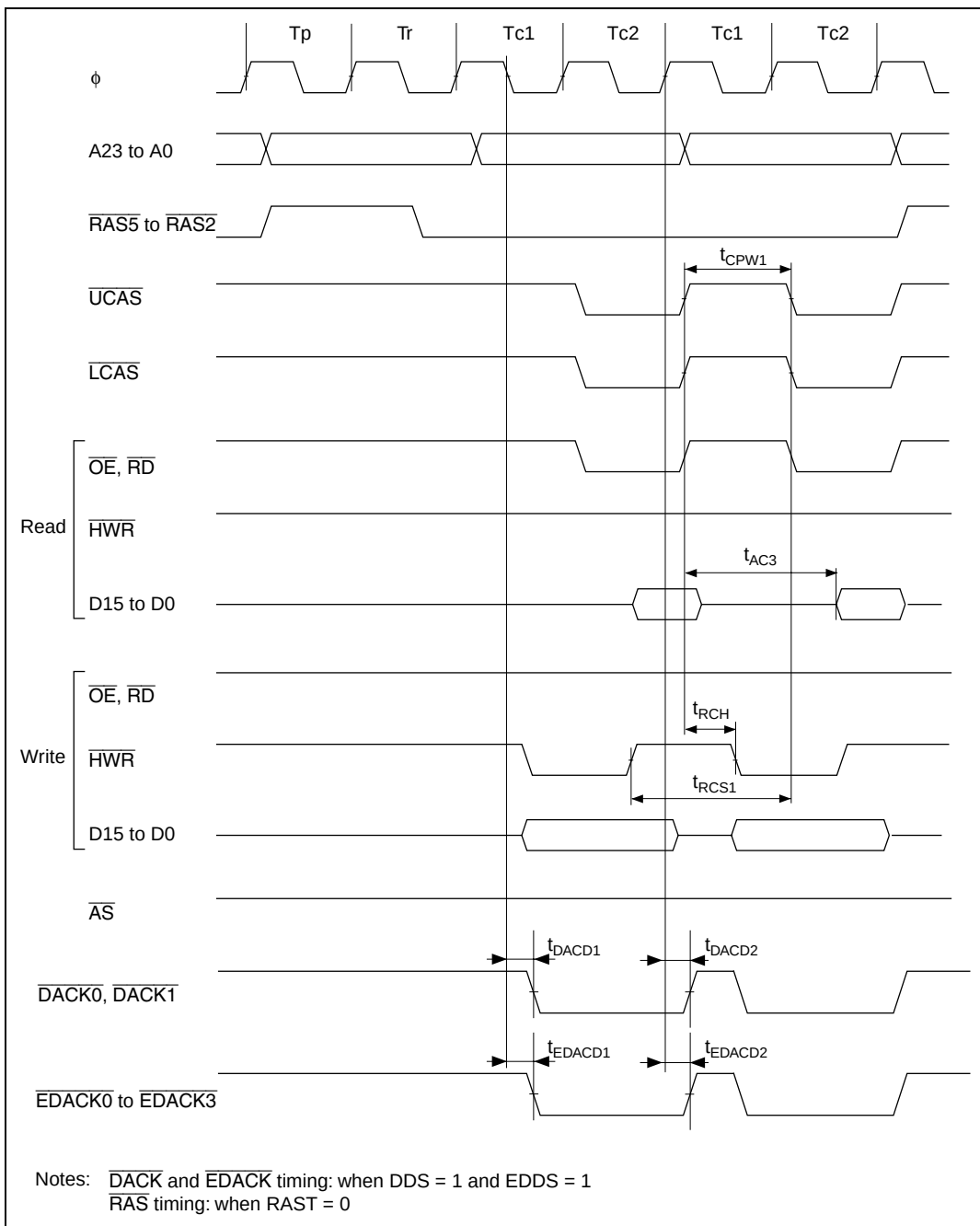
Figure 24.16 DRAM Access Timing: Two-State Burst Access
