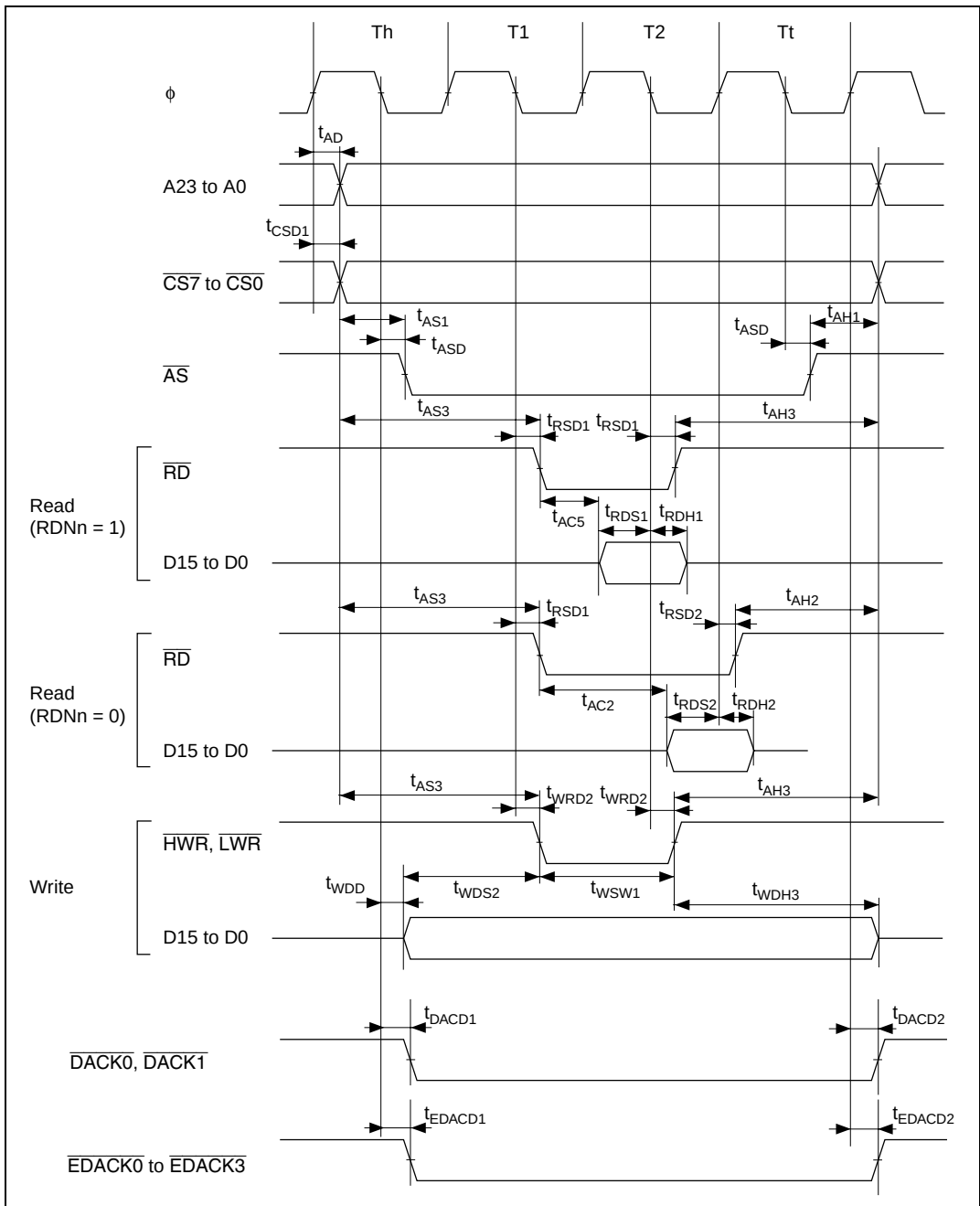
Figure 24.10 Basic Bus Timing: Two-State Access ( \overline{\text{CS}} Assertion Period Extended)
