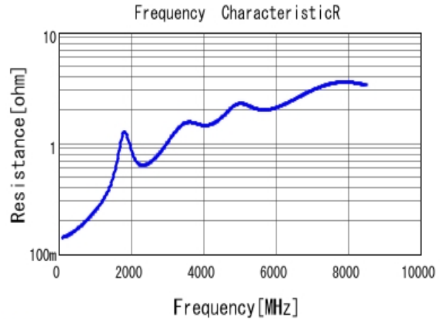
■ GRM1885C2A680JA01 R DC0V, 25degC
