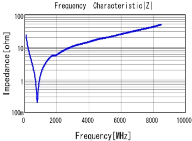
■ GRM1885C2A680JA01 |Z| DC0V, 25degC
