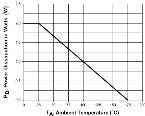
Power Derating
