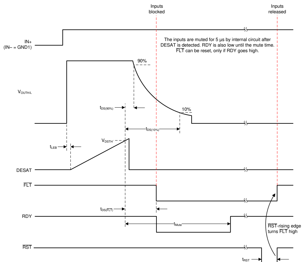
Figure 8-3. DESAT, OUTH, OUTL, \overline{\text{FLT}} , \overline{\text{RST}} Delay
