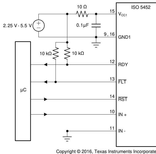
Figure 10-4. \overline{\text{FLT}} and RDY Pin Circuitry for High CMTI
