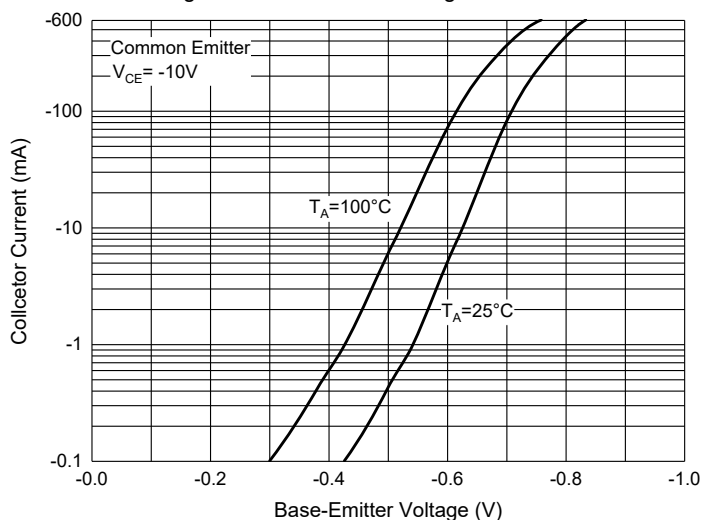
Fig. 11 - Base-Emitter Voltage Characteristics
