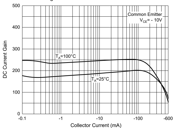
Fig. 8 - DC Current Gain Characteristics
