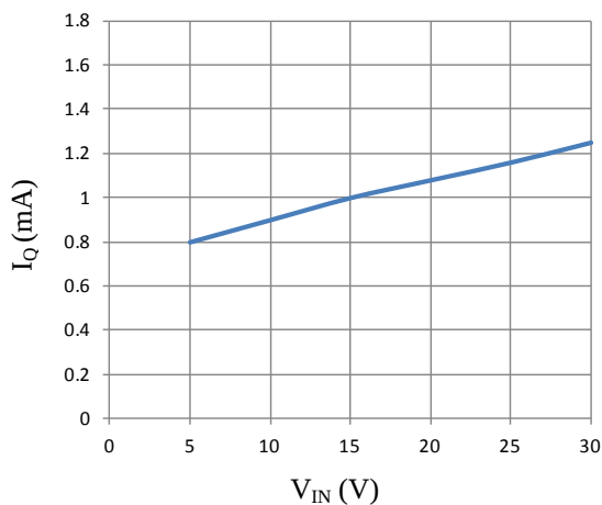
Figure 5-1. Quiescent Current, I_Q vs. Input Voltage, V_{IN}
