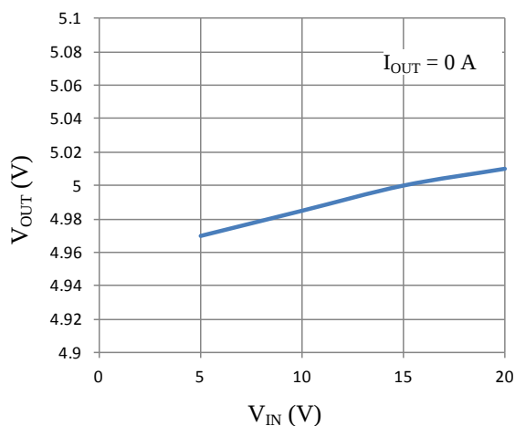
Figure 5-4. Line Regulation
