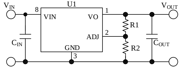
Figure 12-1. ADJ Pin Peripheral Circuit
