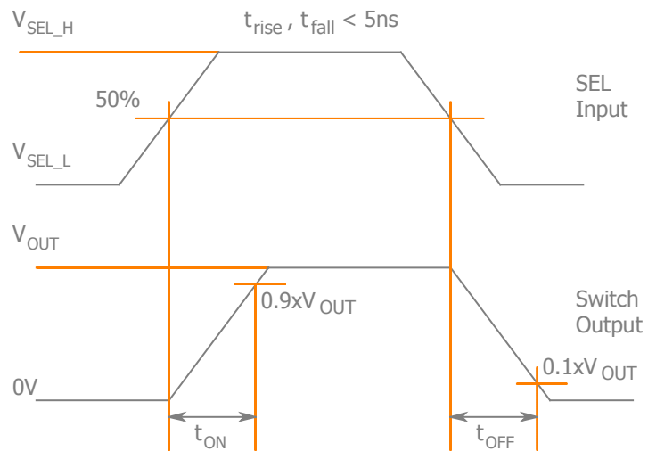
Figure 1. t_{ON} , t_{OFF}
