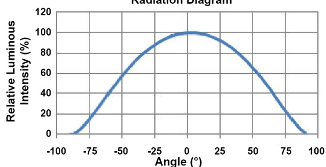
Radiation Diagram
