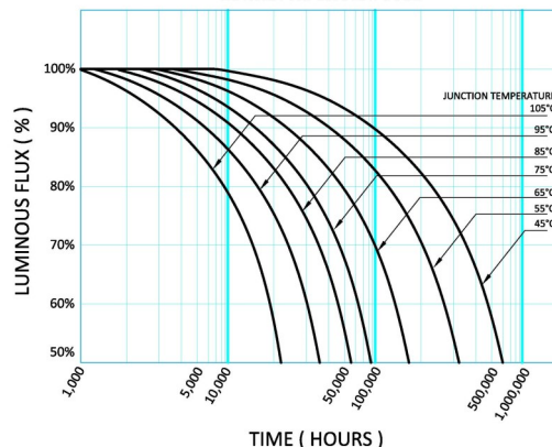
LUMEN MAINTENANCE
