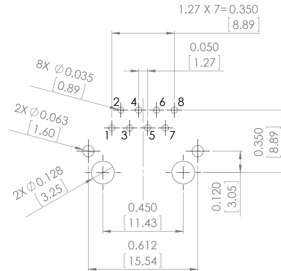
Recommended Hole Pattern View From Component Side
