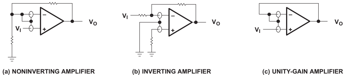
Figure 40. Guard-Ring Schemes
