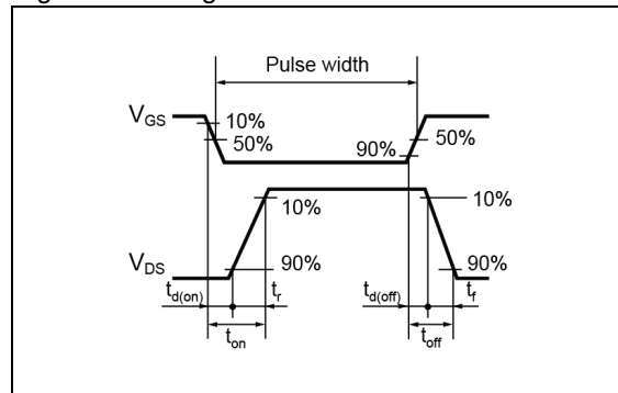
Fig.1-2 Switching Waveforms
