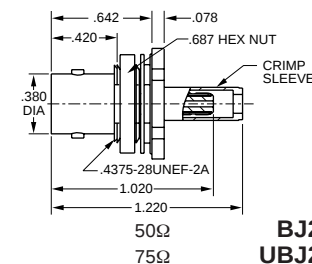
BULKHEAD CABLE JACK REAR MOUNT, TOOL CRIMP
