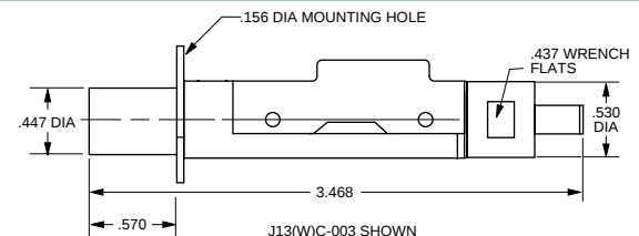
PATCH JACK SELF-TERMINATING
