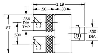
ADAPTER FIXED PARALLELING 50Ω TPS - ONE JACK, TWO PLUGS
