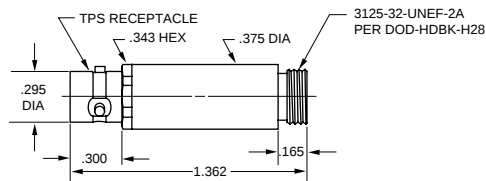
MINIATURE PATCH JACK TPS JACK
