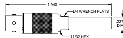
ADAPTER 50Ω MINIATURE PATCH PLUG TO 50Ω TPS JACK .... ADM1
