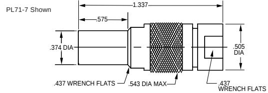
PATCH PLUG
