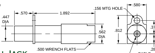
PATCH JACK CABLE ENTRY
