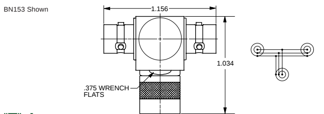
"T" ADAPTER
