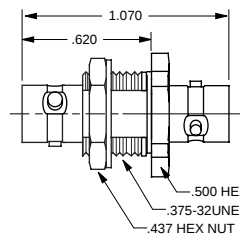
FEED-THROUGH JACK
