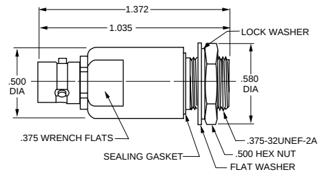
FEED THRU BULKHEAD MOUNT MINIATURE PATCH JACK
