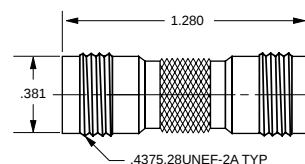
TNC COUPLING ADAPTER (BARREL CONNECTOR)
