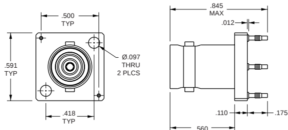
COAX BNC SURFACE MOUNT COMPLIANT TAIL & MOUNT LEGS STRAIGHT
