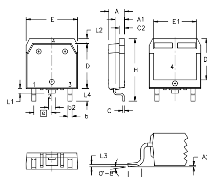
TO-268 Outline
