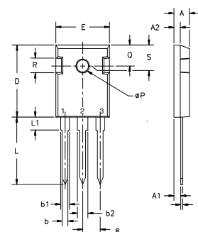
TO-247 AD Outline
