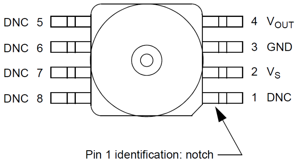
Figure 2. Device pinout (top view)
