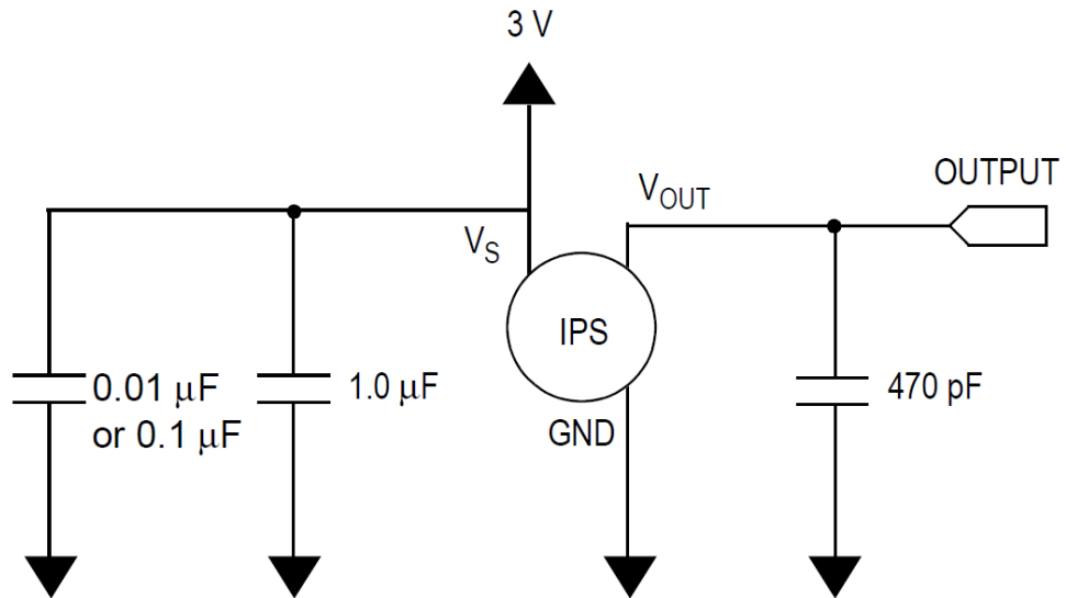
Figure 4. Recommended power supply decoupling and output filtering
