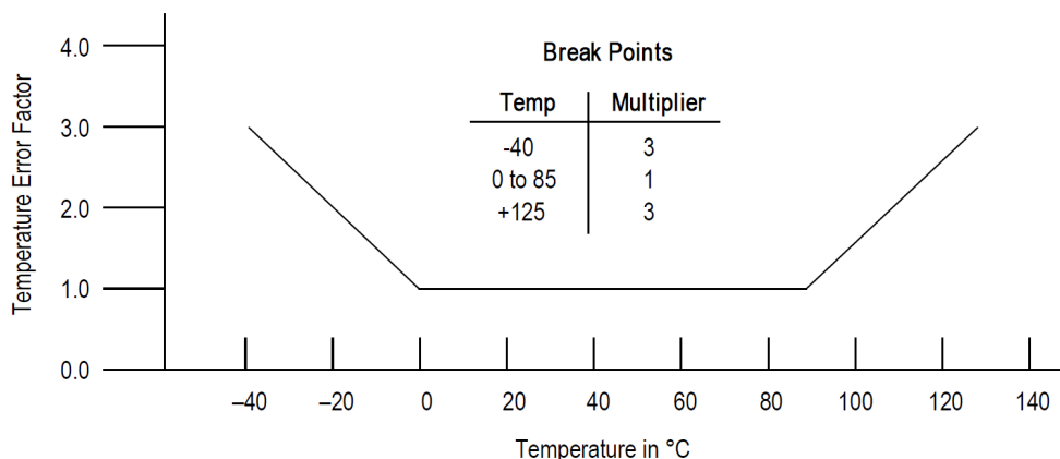
Figure 7. Temperature error band
