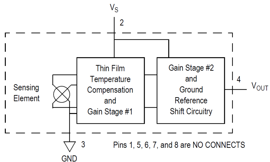
Figure 1. Fully integrated pressure sensor block diagram
