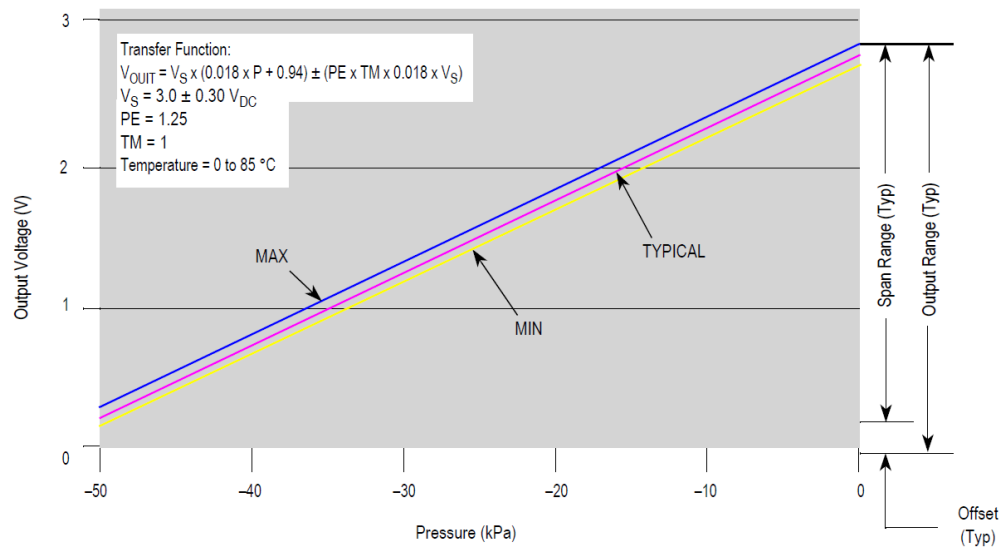
Figure 6. Transfer function
