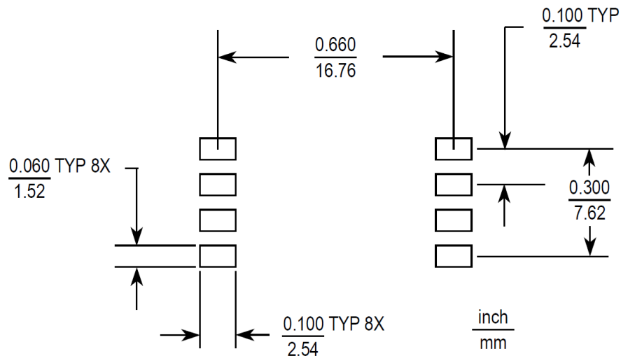
Figure 9. SOP footprint
