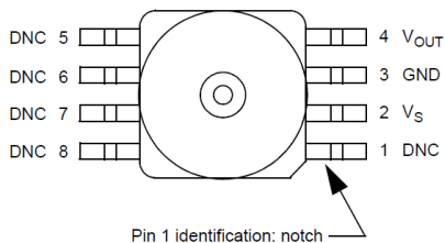
MP3V5050V Case 98ASB17757C
