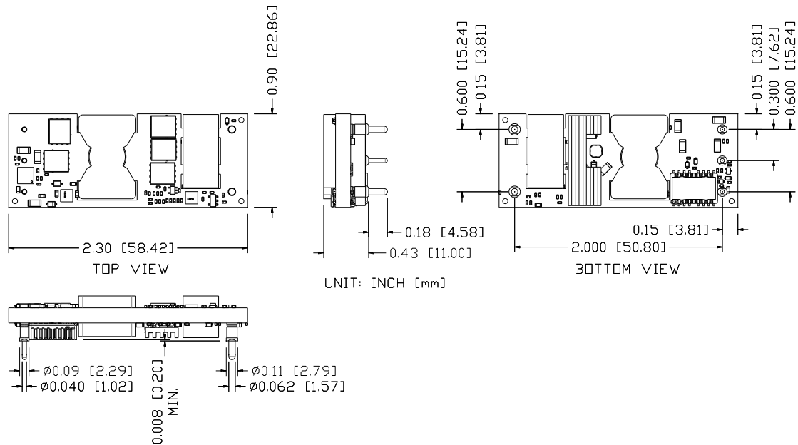
Figure 30. ORCY-T0T120/L Outline
