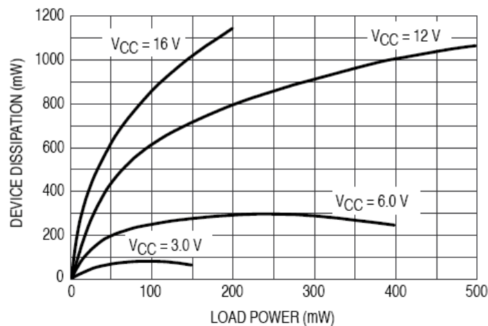
Figure 10. Device Dissipation, 32Ω Load
