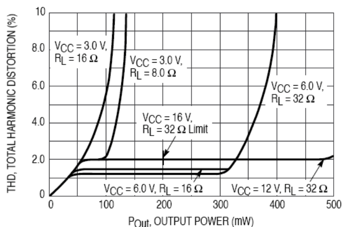
Figure 12. Distortion vs. Power (f=3kHz, AVD=34dB)
