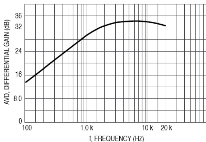
Figure 23. Frequency Response of Figure 22
