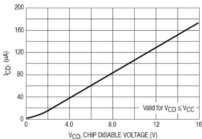
Figure 20. Input Characteristics @ CD (Pin1)
