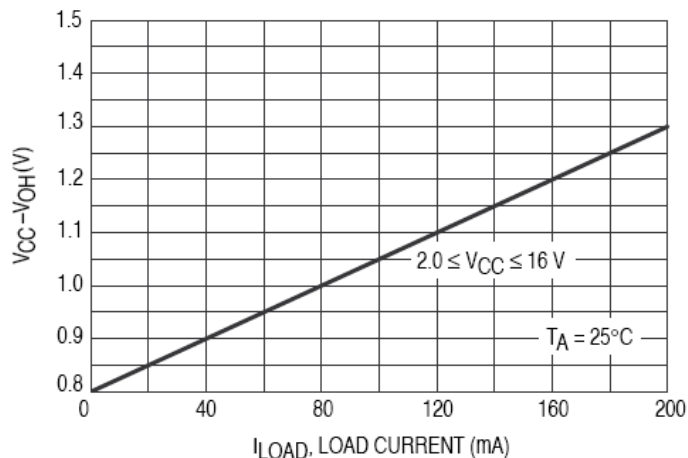
Figure 18. Vcc-Voh @ Vo1, Vo2 vs. Load Current
