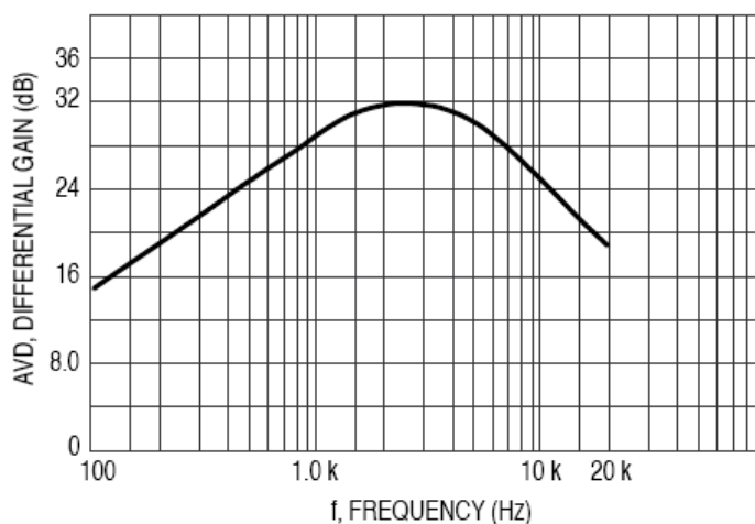
Figure 25. Frequency Response of Figure 24
