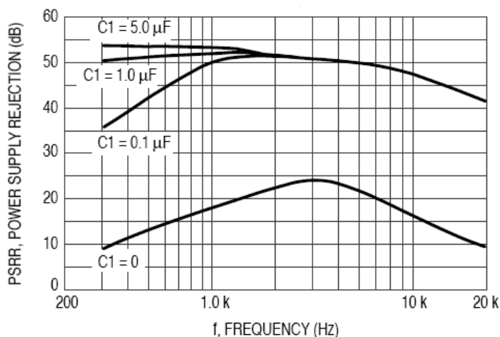
Figure 6. PSRR vs. Frequency (C2=1uF)
