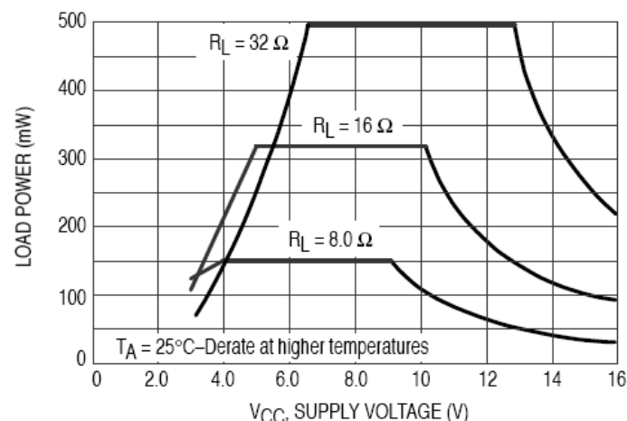
Figure 14. Maximum Allowable Load Power
