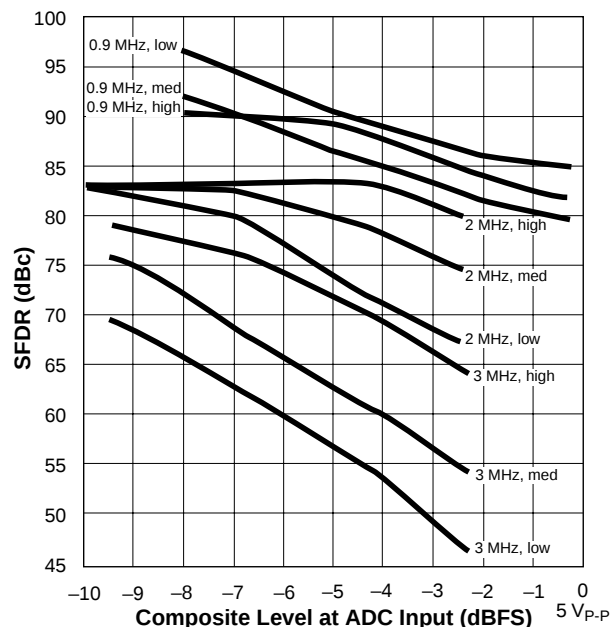
Spurious-Free Dynamic Range
