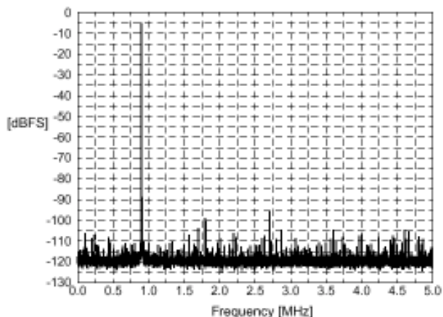
FFT Plot
