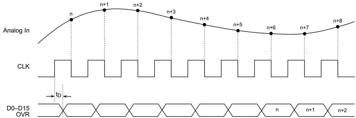
Figure 3 – Timing Diagram 1
