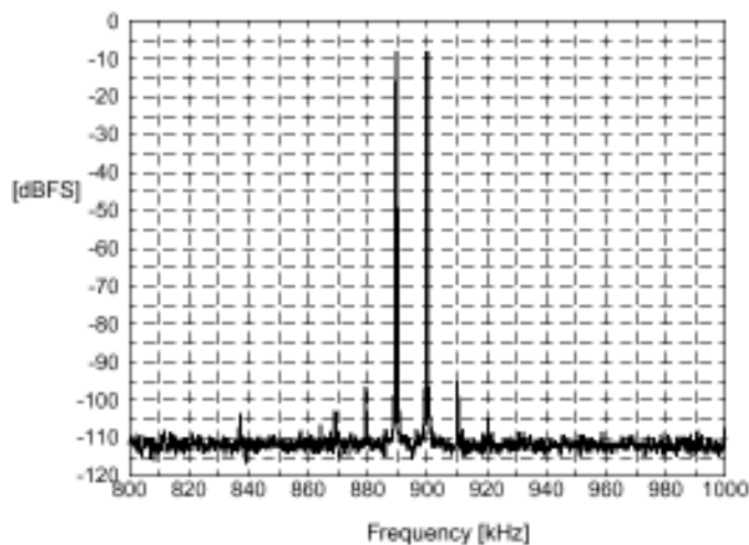
Two-Tone Intermodulation FFT
