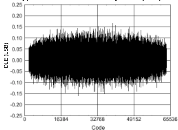
Typical Differential Linearity Error (DLE)
