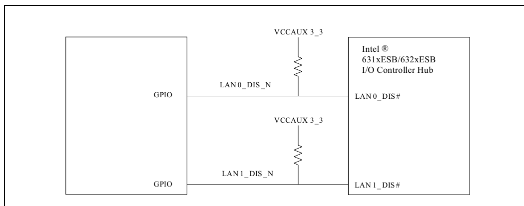
Figure 5-10. LAN Port Disable
