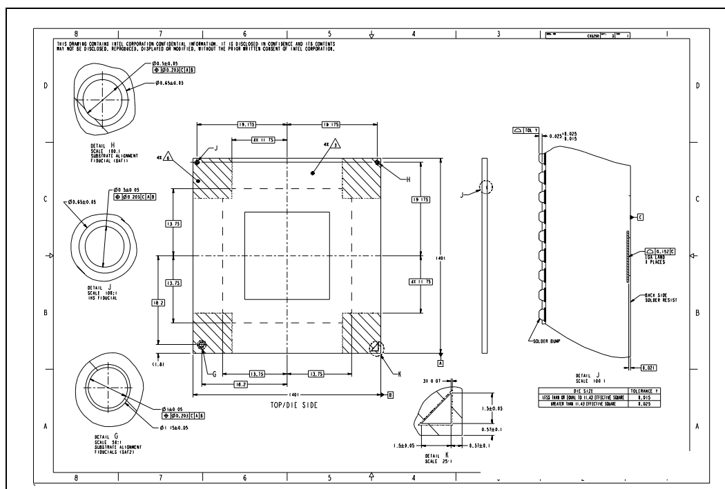
Figure 9-2. Mechanical Layout
