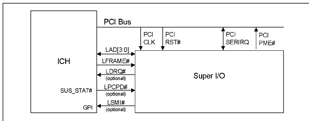
Figure 5-14. LPC Interface Diagram
