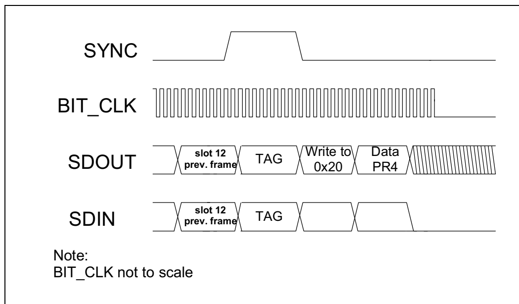
Figure 5-38. AC-Link Powerdown Timing
