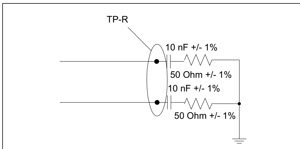
Figure 6-5. Kumeran Receive Test Point (TP-R)
