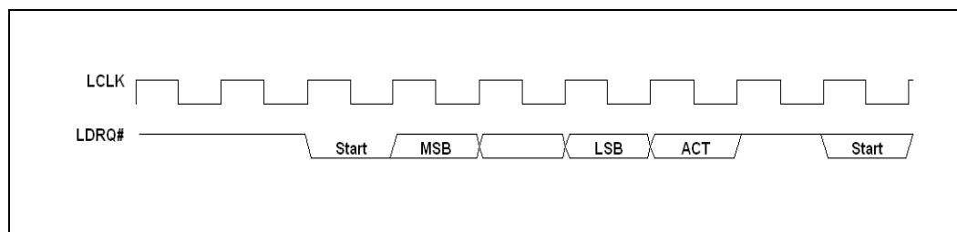
Figure 5-16. DMA Request Assertion through LDRQ#
