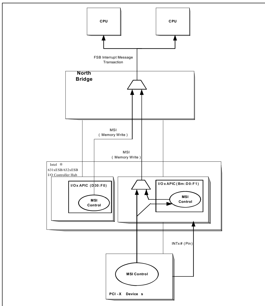
Figure 5-6. System Interrupt Architecture
