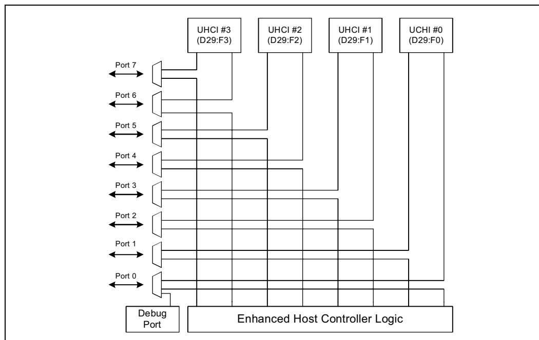
Figure 5-23. Intel® 631xESB/632xESB I/O Controller Hub-USB Port Connections
