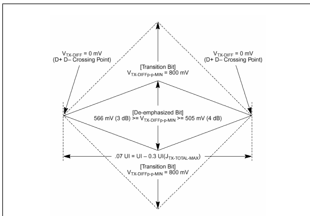
Figure 6-2. Minimum Transmitter Timing and Voltage Output Compliance Specification
