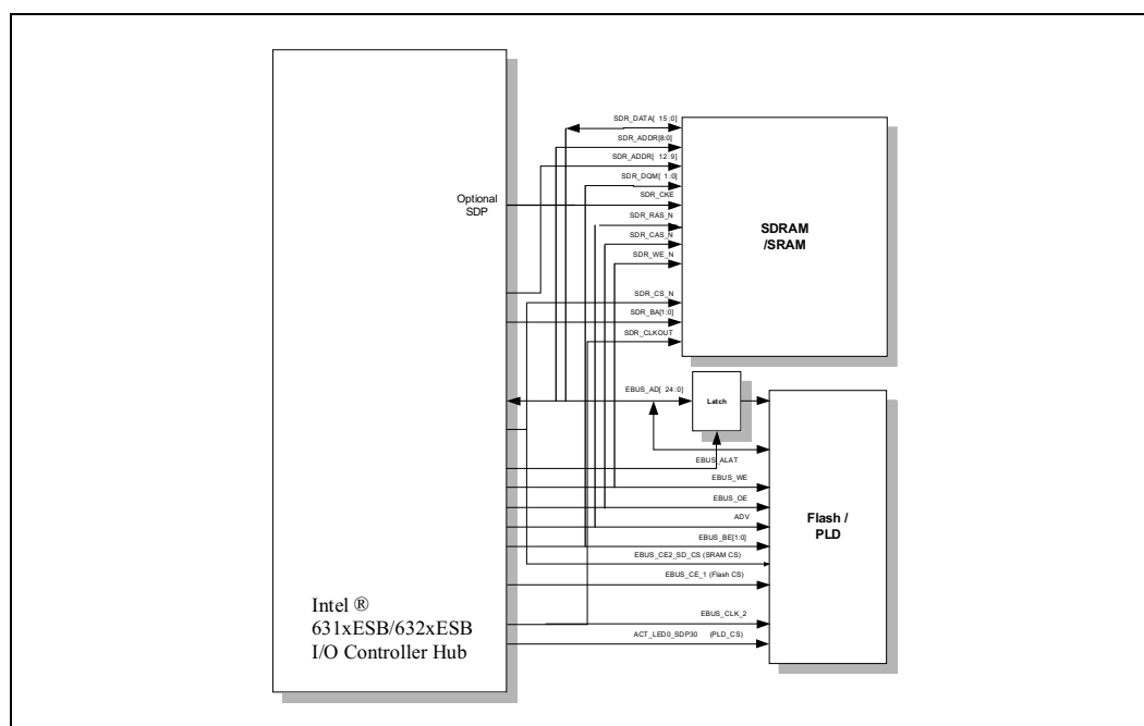
Figure 5-13. Expansion Bus Signal Block Diagram
