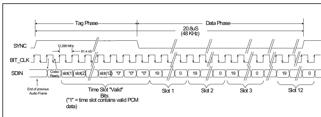
Figure 5-37. AC-Link Protocol
