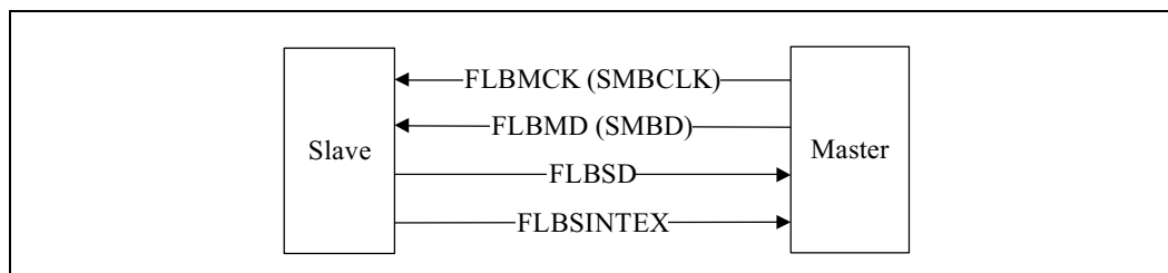
Figure 5-11. FML Topology
