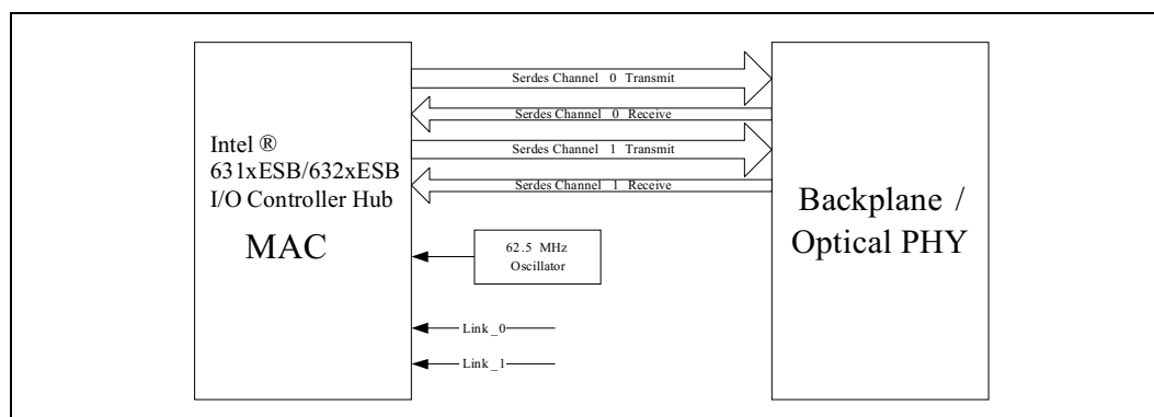
Figure 5-9. SerDes Backplane Connection
