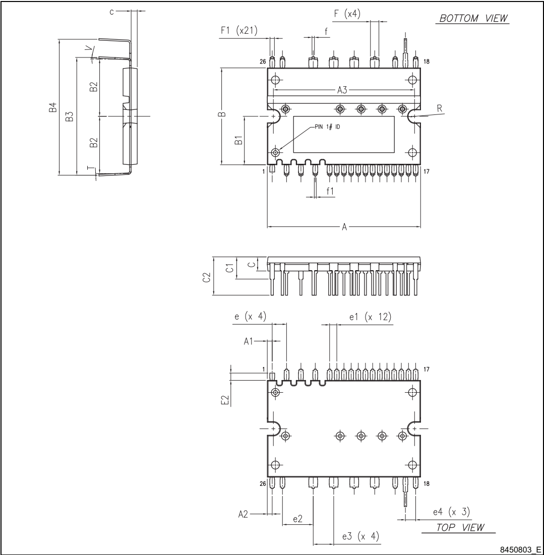
Figure 17. SDIP2F-26L type E package outline
