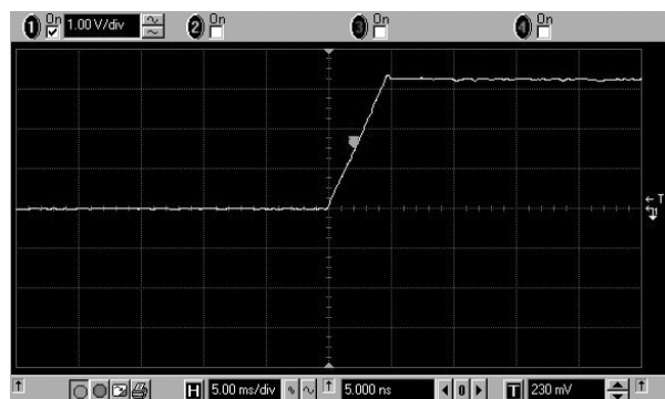
Rise Time
