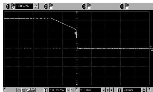
Fall Time
