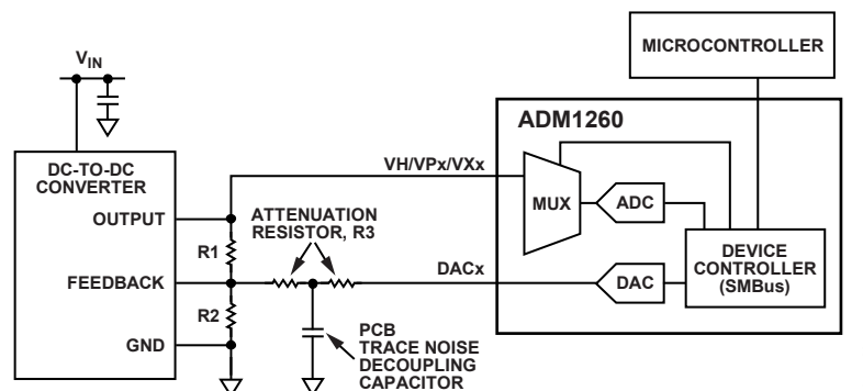
Figure 34. Closed-Loop Margining System Using the ADM1260
