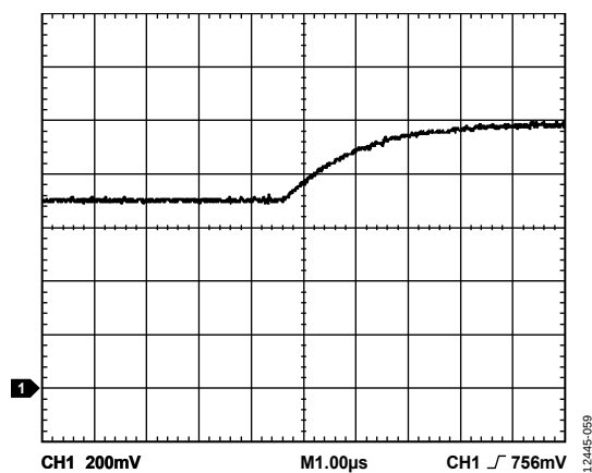
Figure 16. Transient Response of the DAC Code Change into a Typical Load (See Figure 20 for the Corresponding Probe Point Diagram)
