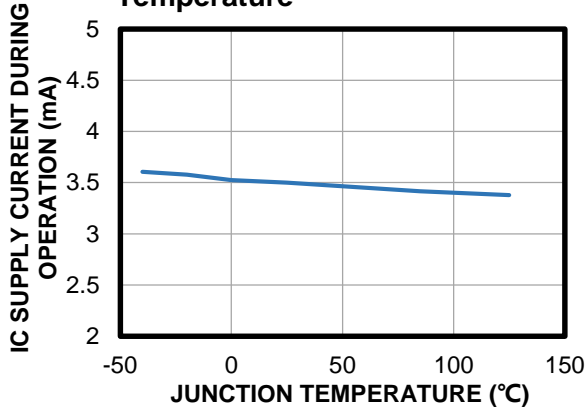
IC Supply Current during Operation vs. Junction Temperature
