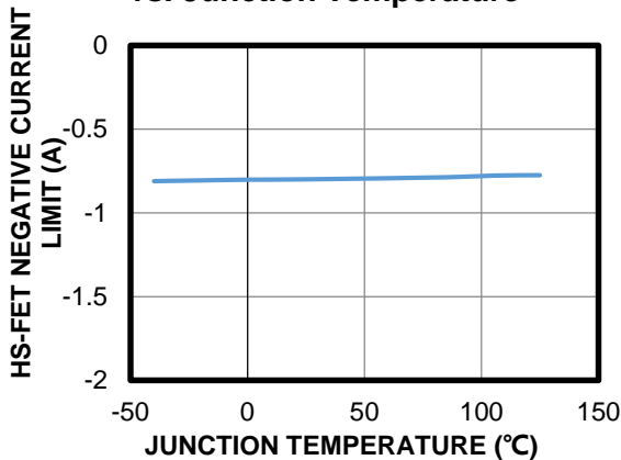
HS-FET Negative Current Limit vs. Junction Temperature
