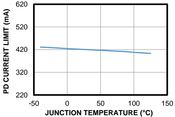
PD Current Limit vs. Junction Temperature
