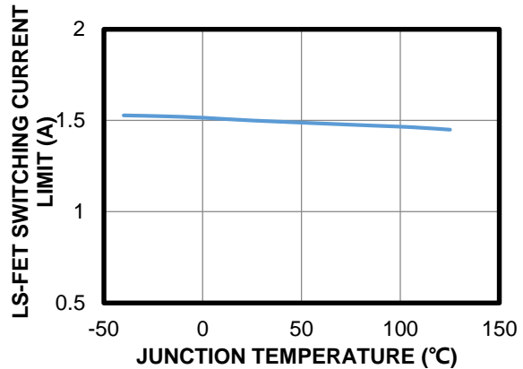
LS-FET Switching Current Limit vs. Junction Temperature
