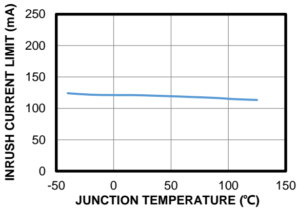
Inrush Current Limit vs. Junction Temperature
