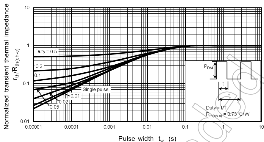
Fig. 9.13 r_{th}/R_{th(ch-c)} - t_w (Guaranteed Maximum)
