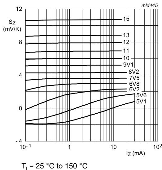
Fig. 7. Per diode: Temperature coefficient as a function of working current; typical values (BZB84-B/C5V1-Q to BZB84-B/C15-Q)
