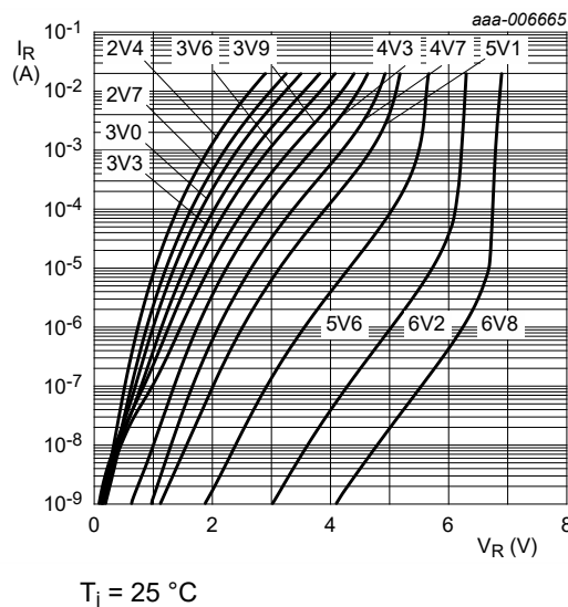
Fig. 8. Per diode: Reverse current as a function of reverse voltage; typical values (BZB84-B/C2V4-Q to BZB84-B/C6V8-Q)
