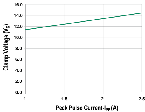
Clamping Voltage vs IPP
