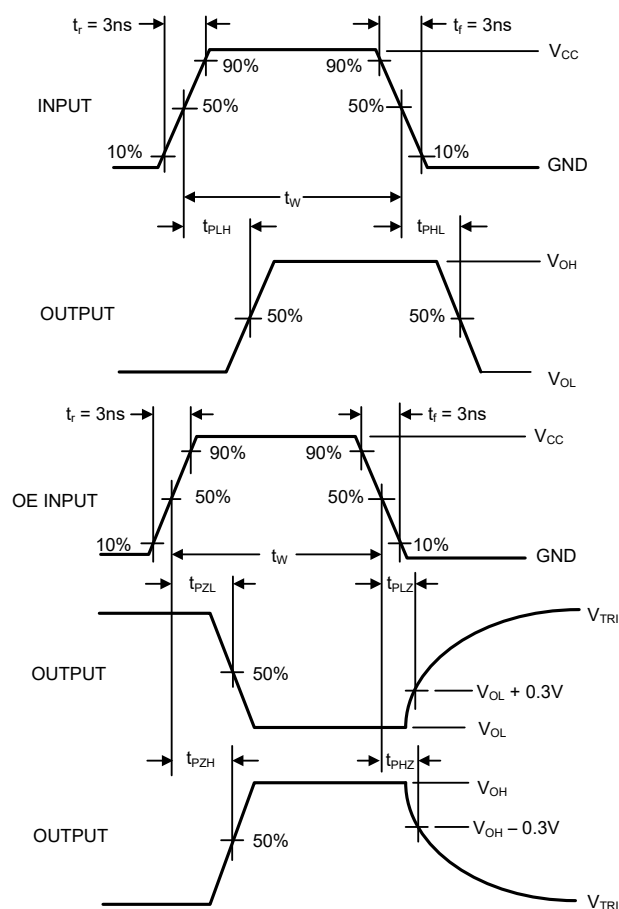
Figure 2. AC Waveforms
