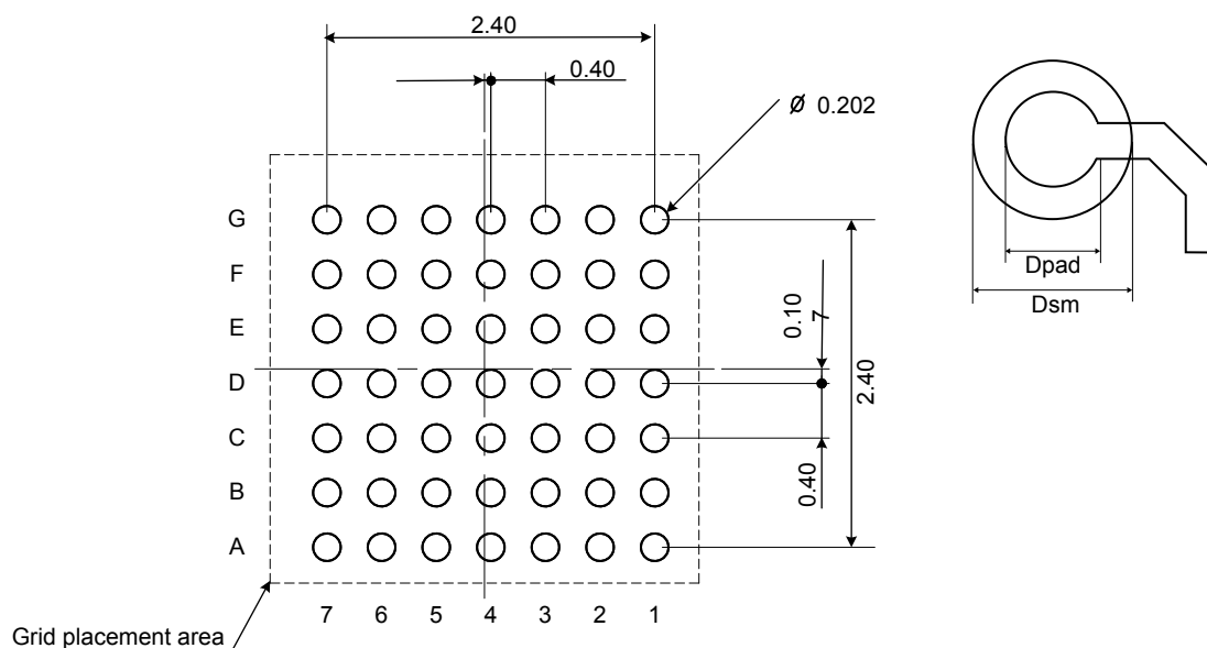
Figure 24. WLCSP49 - Footprint example
