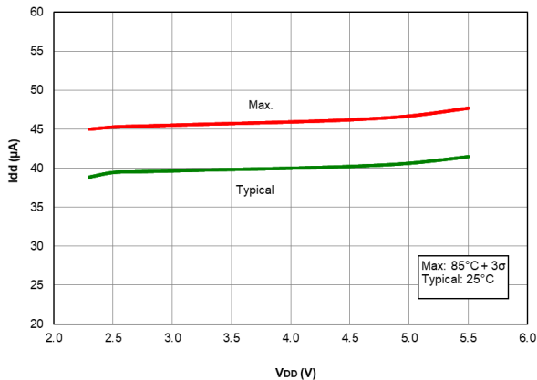
Figure 40-5. I_{PD} Fixed Voltage Reference (FVR) PIC16F18425/45 only
