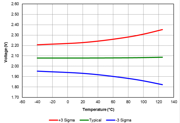
Figure 40-44. LPBOR Reset Voltage, All devices
