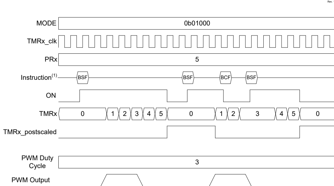
Figure 20-7. Software Start One Shot Mode Timing Diagram (MODE = 01000)
