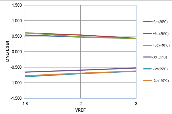
Figure 40-56. ADC 12-Bit Mode, Single-Ended DNL, V_{DD} = 3.0V , T_{AD} = 1 \mu s , All devices
