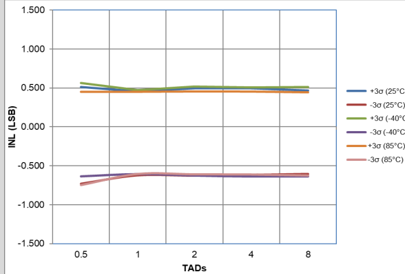
Figure 40-55. ADC 12-Bit Mode, Single-Ended INL, V_{DD} = 3.0V , V_{REF} = 3.0V , All devices
