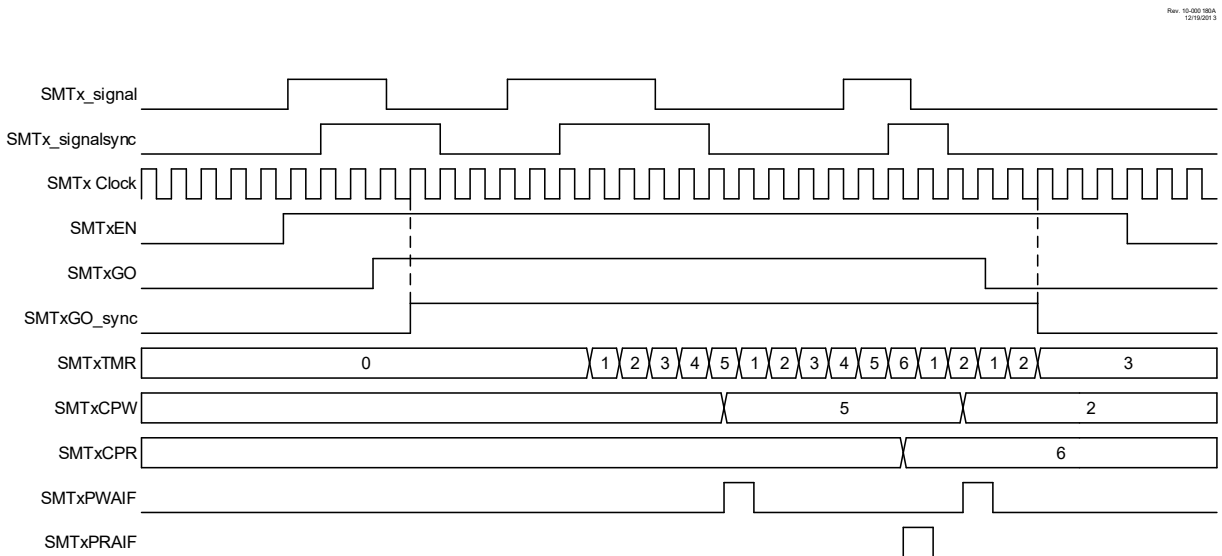
Figure 21-7. High and Low Measurement Mode, Repeat Acquisition Timing Diagram
