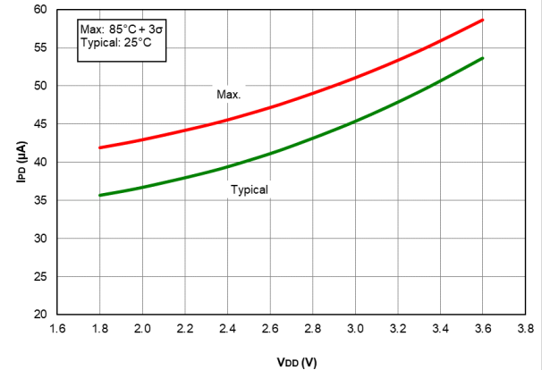
Figure 40-6. I_{PD} Brown-Out Reset (BOR), BORV = 1 PIC16LF18425/45 only
