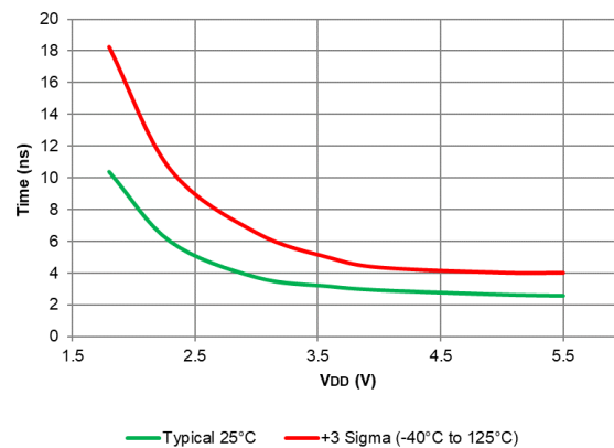
Figure 40-102. Fall Time, Slew Rate Control Disabled, All devices
