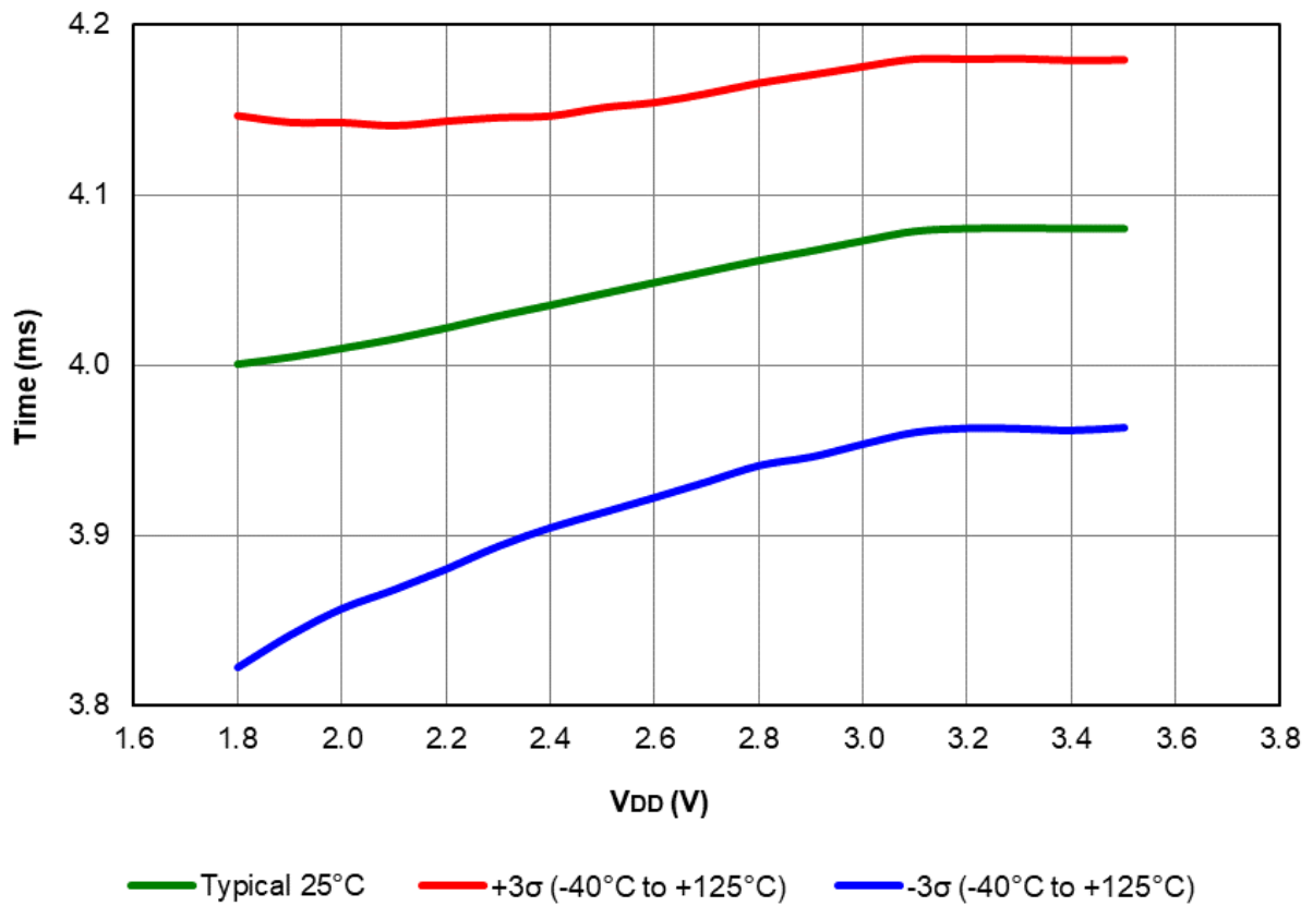
Figure 40-115. WDT Time-Out Period, PIC16LF18425/45 only
