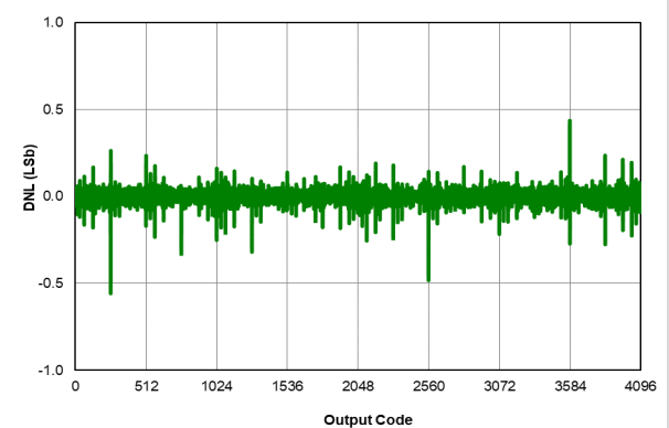
Figure 40-48. ADC 12-Bit Mode, Single-Ended Typical DNL, V_{DD} = 3.0V , V_{REF} = 3.0V , T_{AD} = 0.5 \mu s , 25°C, All devices
