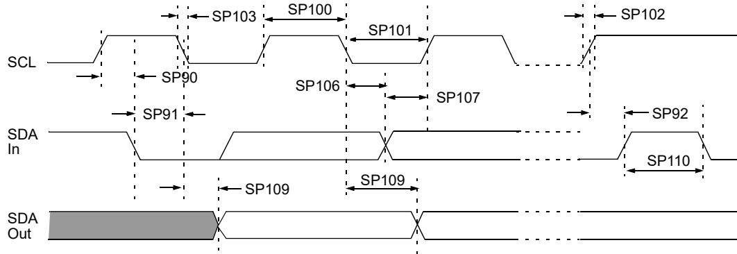
Figure 39-22. I 2 C Bus Data Timing
