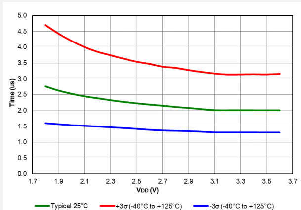
Figure 40-66. ADC RC Oscillator Period, PIC16LF18425/45 only
