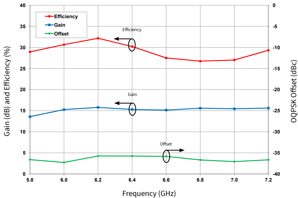
Figure 2. Typical Gain, Efficiency and OQPSK Performance vs Frequency
