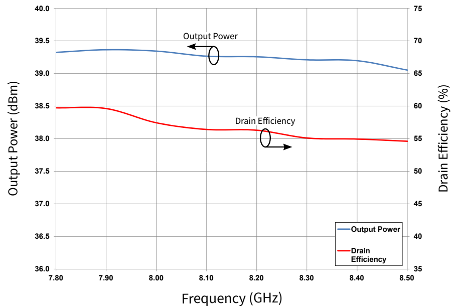
Figure 8. Typical Pulsed Power Response V_{DD} = 40\text{ V} , I_{DQ} = 60\text{ mA} , 100\text{ }\mu\text{s} , 10% Duty, P_{IN} = 28\text{ dBm}
