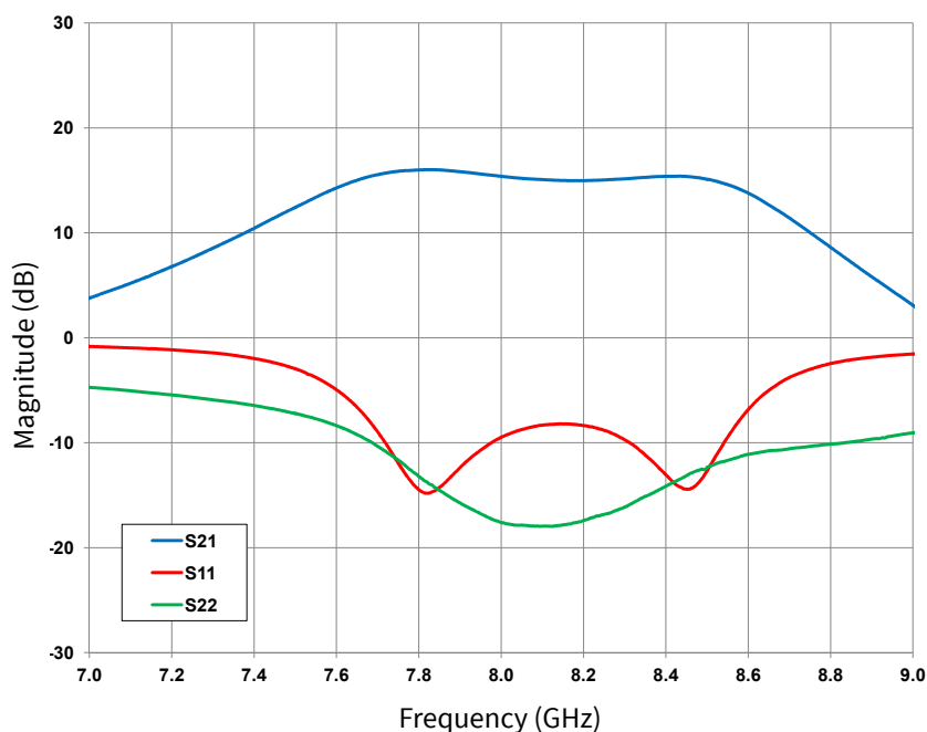
Figure 5. Typical Small Signal Response of CGHV1F006S-AMP2 Application Circuit
