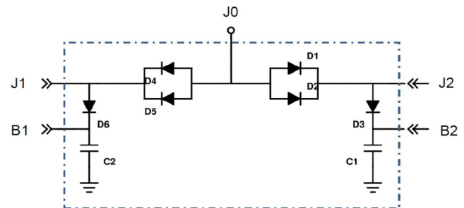
Figure 1 TDSW002040X-198 Schematic
