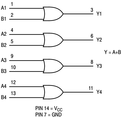
LOGIC DIAGRAM
