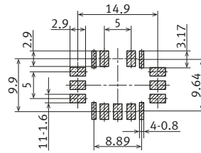
Recommended PC board pattern ( TOP VIEW )
