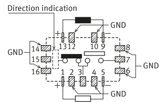
2 coil latching Standard contact ( Reset )
