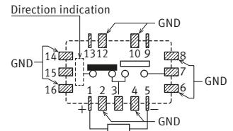
Reverse contact ( De-energize )
