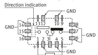
2 coil latching Standard contact ( Reset )
