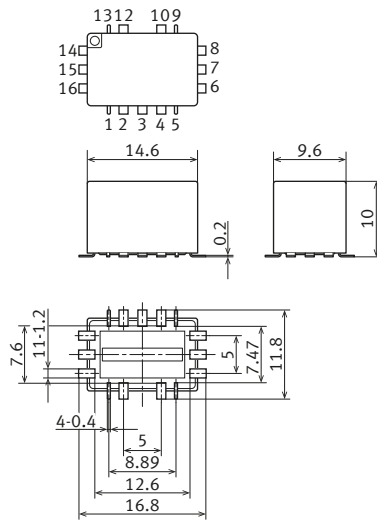
External dimensions
