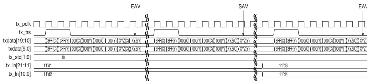
Figure 3–32. Behavior of tx_std, tx_trs, and tx_In Signals—425MB
