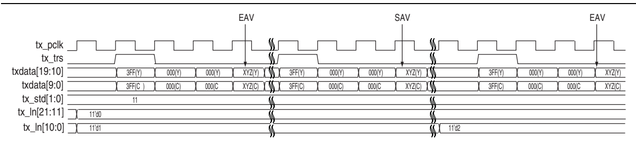
Figure 3-31. Behavior of tx_std, tx_trs, and tx_ln Signals—425MA
