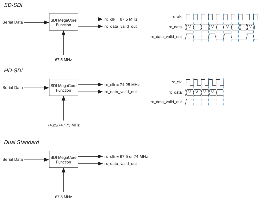
Figure 3-9. Receiver Clocks
