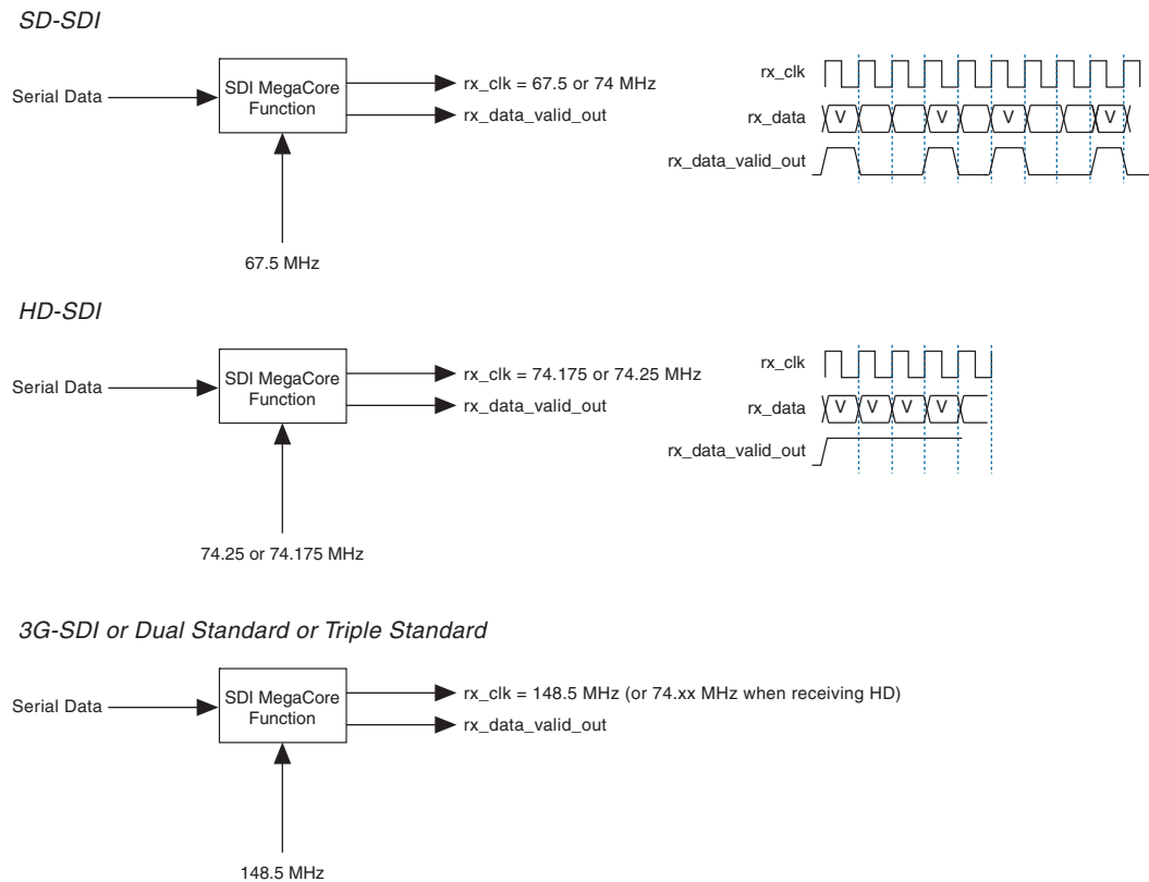
Figure 3-12. Receiver Clocks
