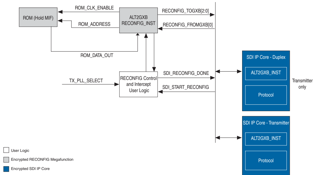
Figure 3–20. Transceiver Dynamic Reconfiguration for Transmitter Clock Multiplexer Block Diagram
