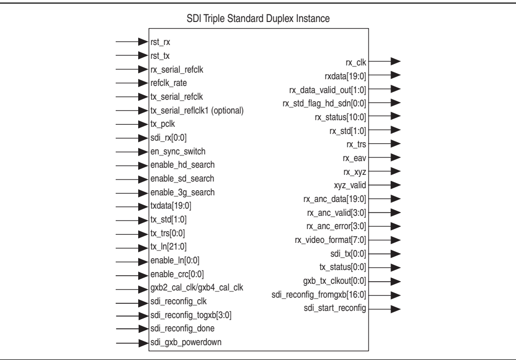
Figure 3-28. Interface Signals for SDI Triple Standard Duplex Instance
