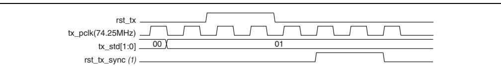
Figure 3-30. Power-up Reset for the Transmitter
