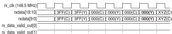
Figure 3–35. Behavior of rx_data_valid Signal—425MB
