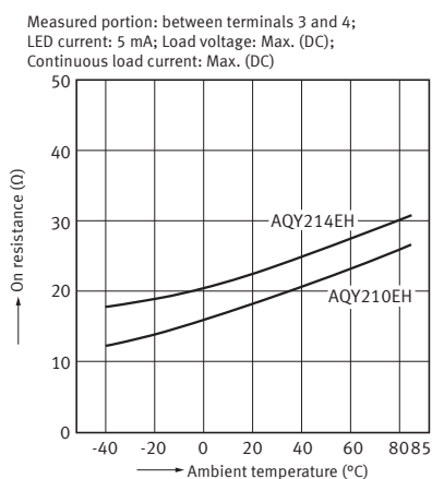
2-1. On resistance vs. ambient temperature characteristics
