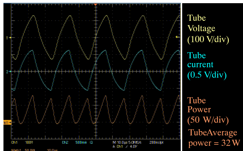
Figure 4. Tube Signals
