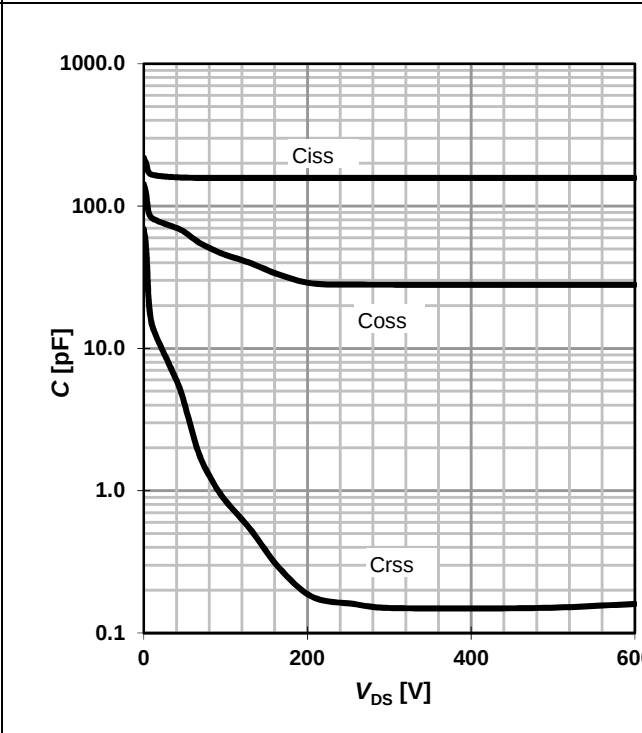
Figure 20 Typ. capacitances
