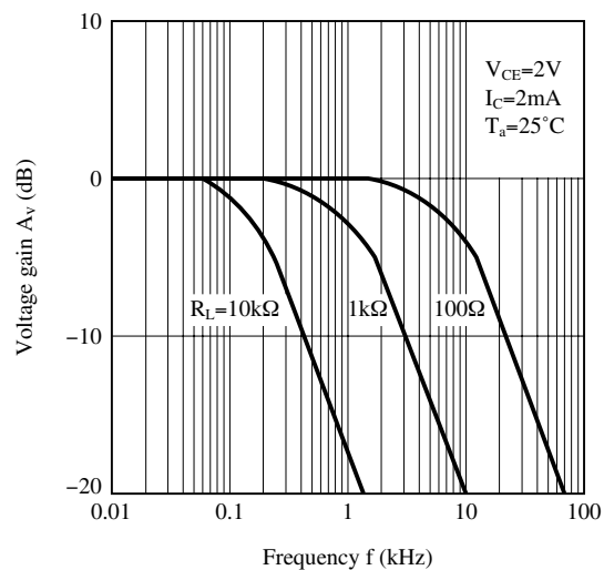
Fig.15 Frequency Response
