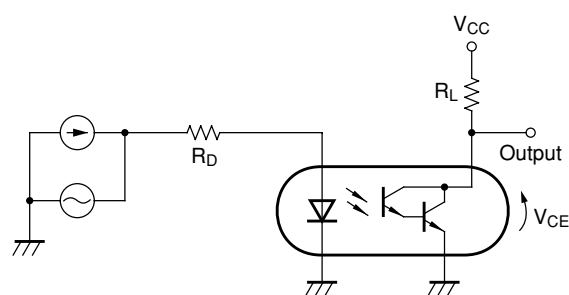
Fig.16 Test Circuit for Frequency Response
