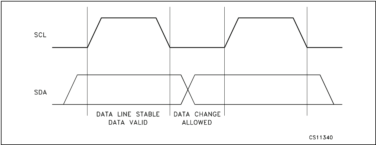
Figure 8. Timing diagram of I 2 C bus
