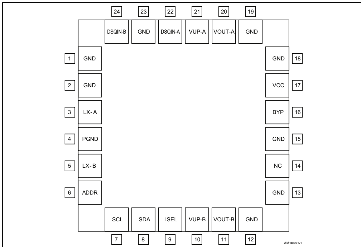
Figure 5. Pin connections (top view)
