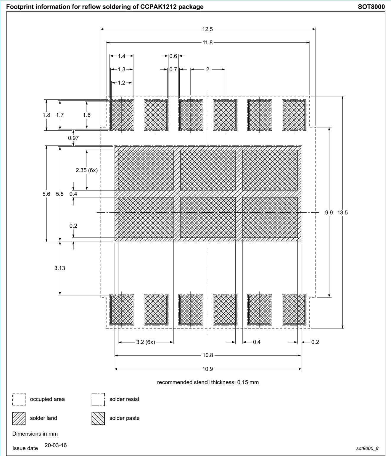
Fig. 6. Reflow soldering footprint for CCPAK (SOT8000)
