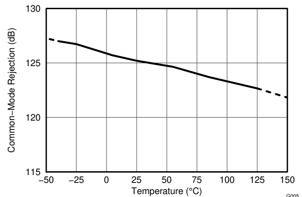
Figure 7-4. Shunt Input Common-Mode Rejection Ratio vs. Temperature
