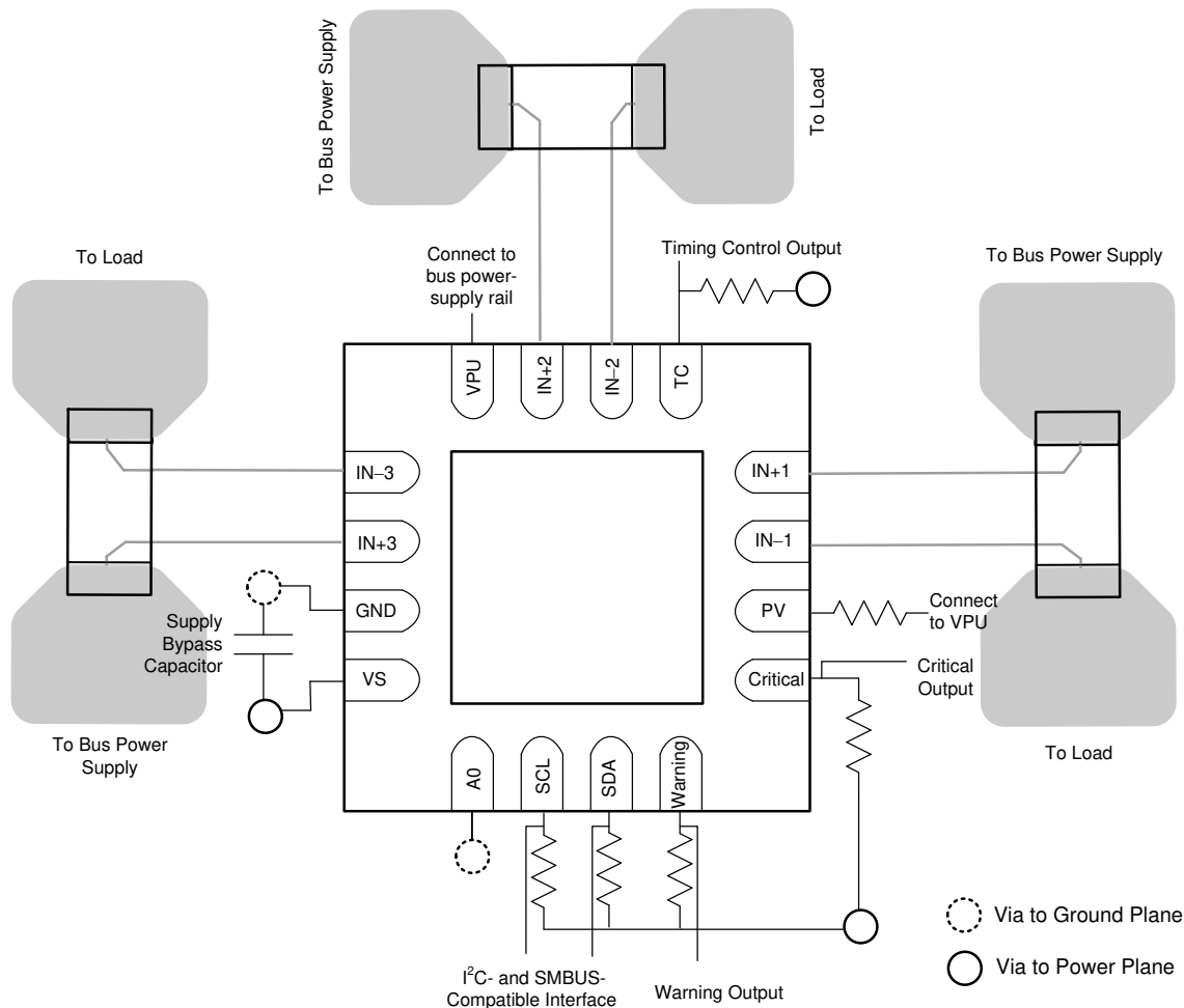
Figure 11-1. Layout Example
