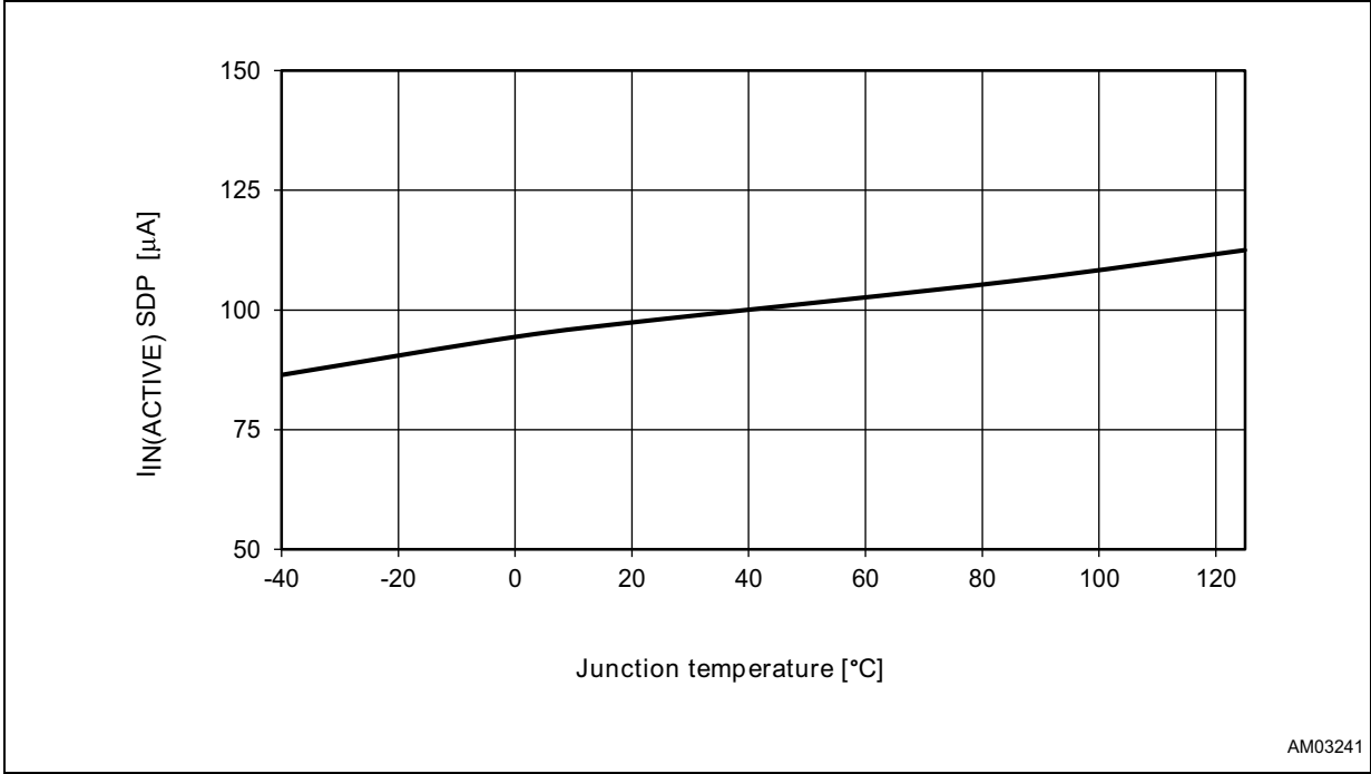
Figure 17. Enabled IN supply current vs. temperature (SDP mode)
