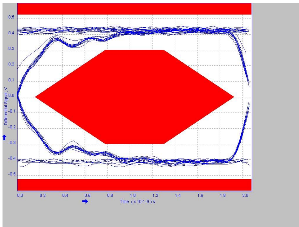
Figure 24. Eye diagram using USB compliance test pattern - with STCC50x1 (STCC50x1 + cable)
