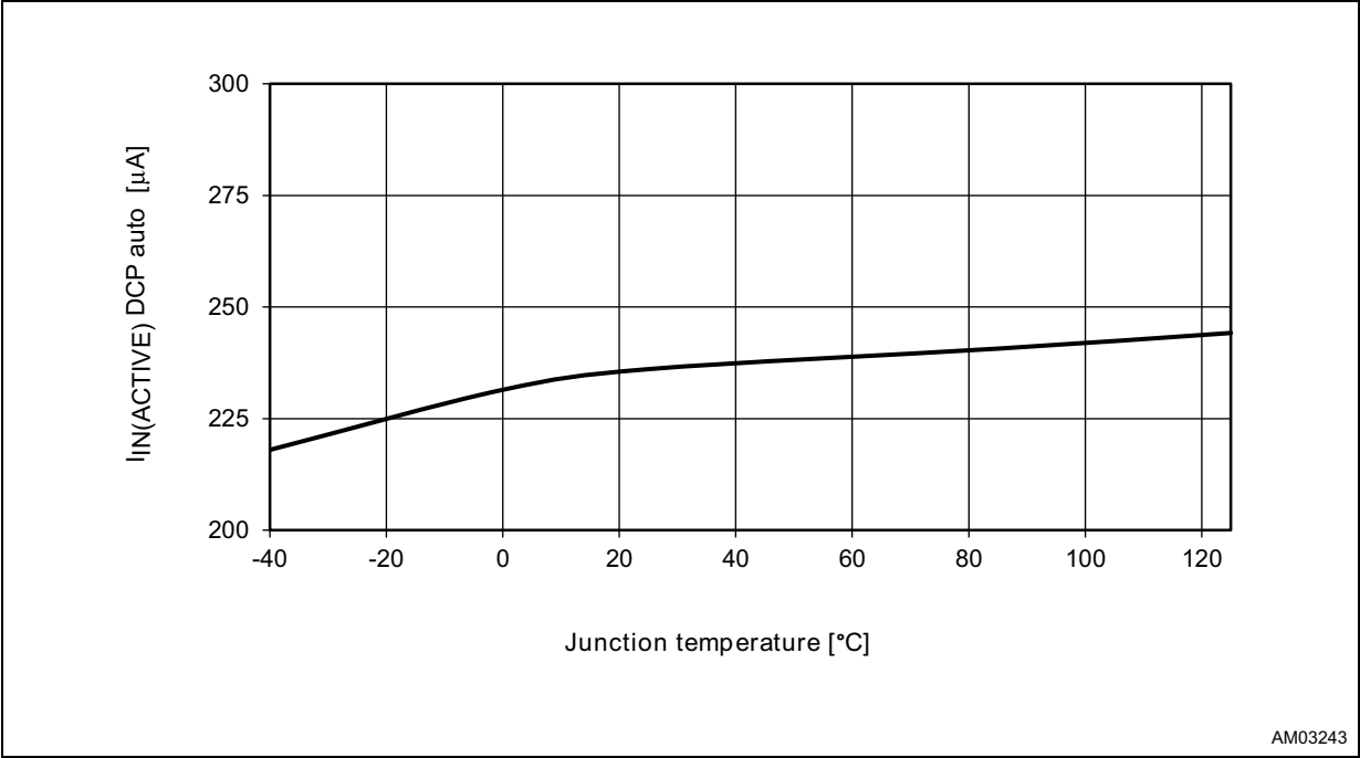
Figure 19. Enabled IN supply current vs. temperature (DCP auto-mode)
