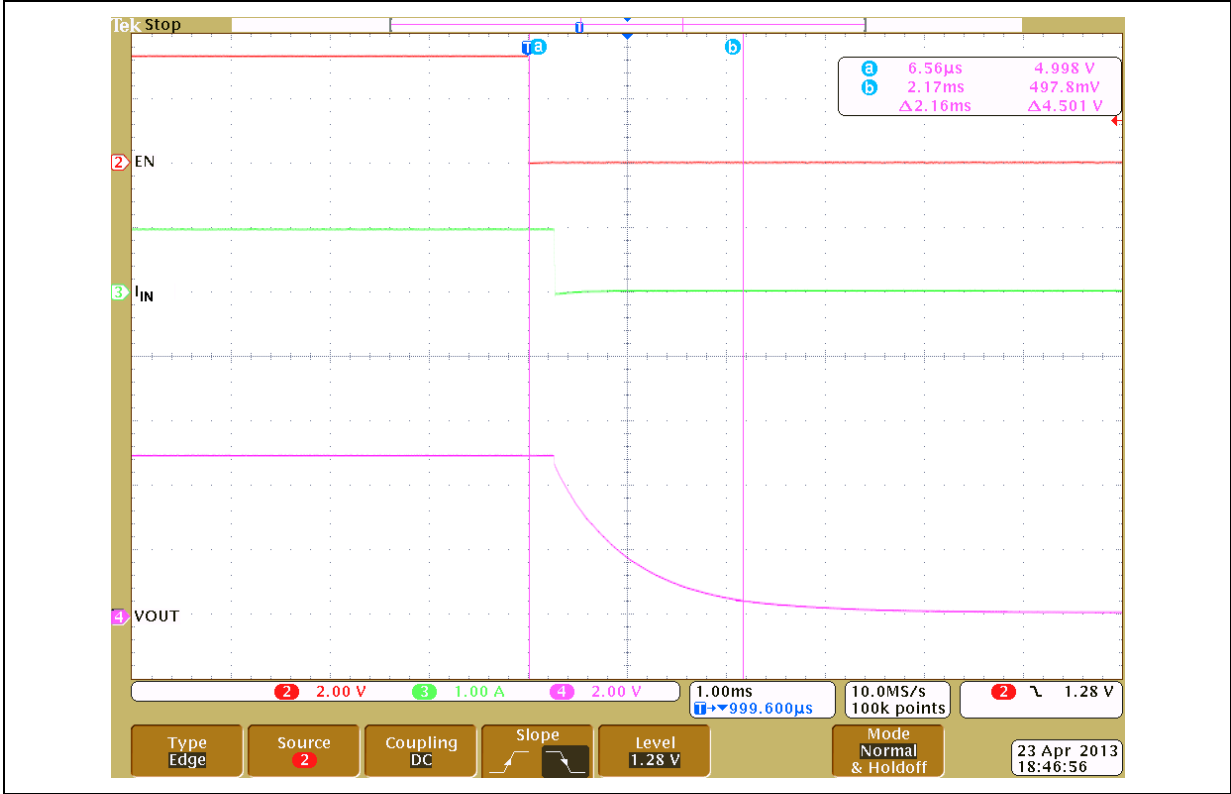
Figure 26. Turn-off response ( R_{LOAD} = 5\text{ }\Omega , C_{LOAD} = 150\text{ }\mu\text{F} )
