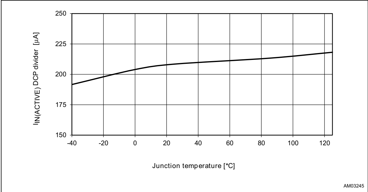
Figure 21. Enabled IN supply current vs. temperature (DCP divider mode)
