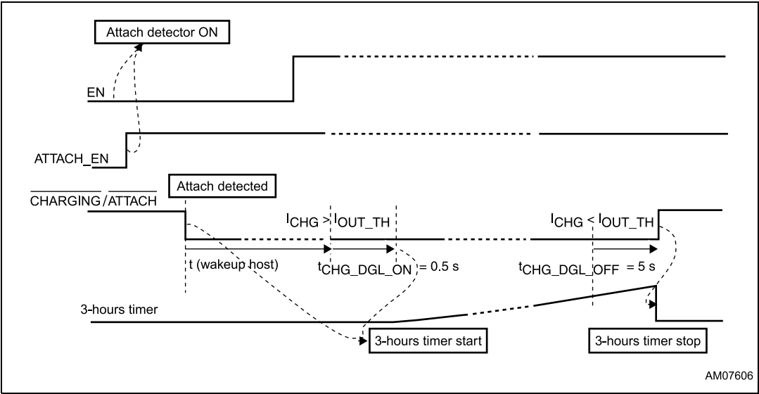
Figure 7. 3-hour timer - start and stop
