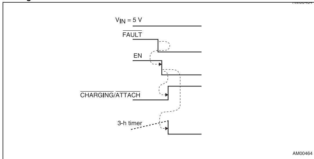
Figure 10. Reset of \overline{\text{CHARGING/ATTACH}} and 3-hour timer after EN \rightarrow 0 event
