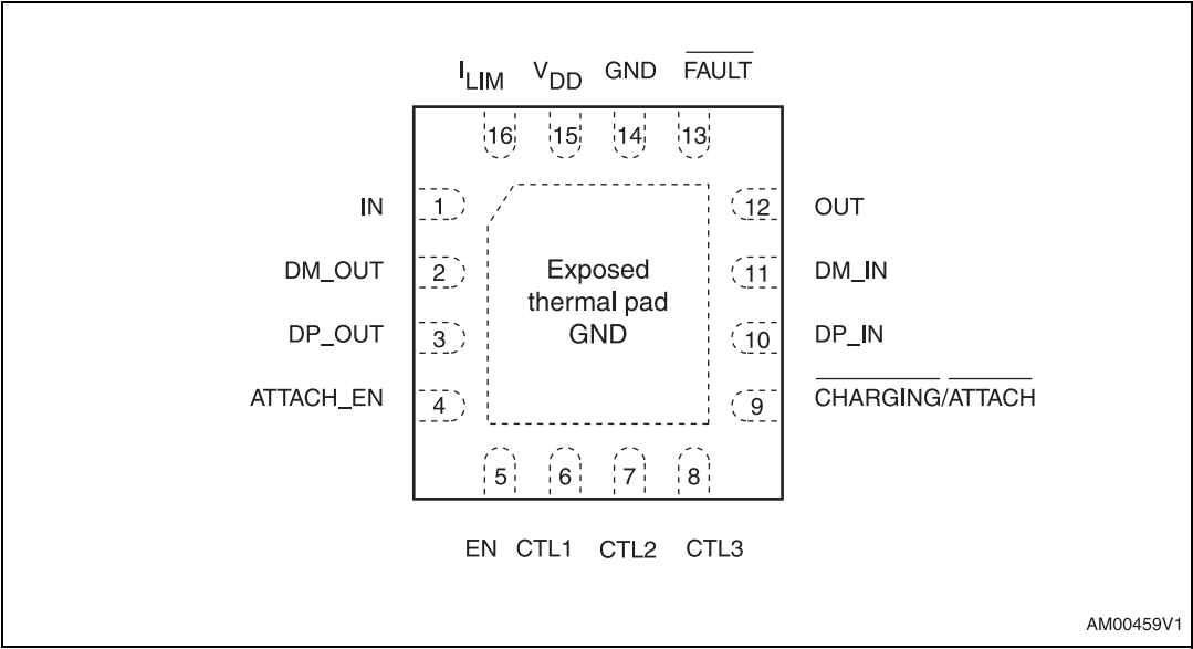
Figure 2. Pinout
