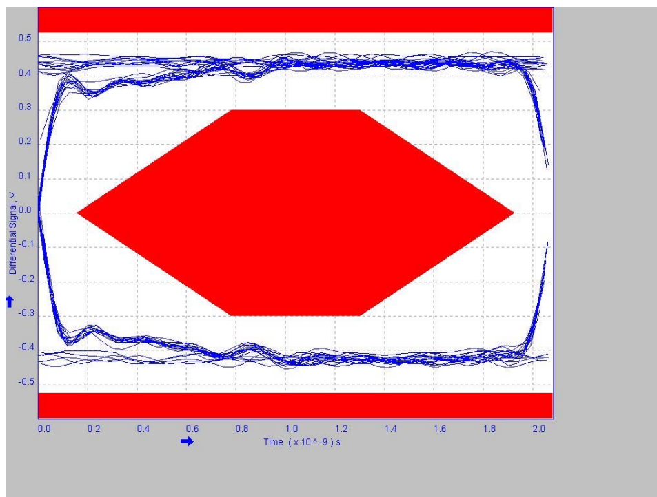
Figure 23. Eye diagram using USB compliance test pattern - without STCC50x1 (deskew line + cable)
