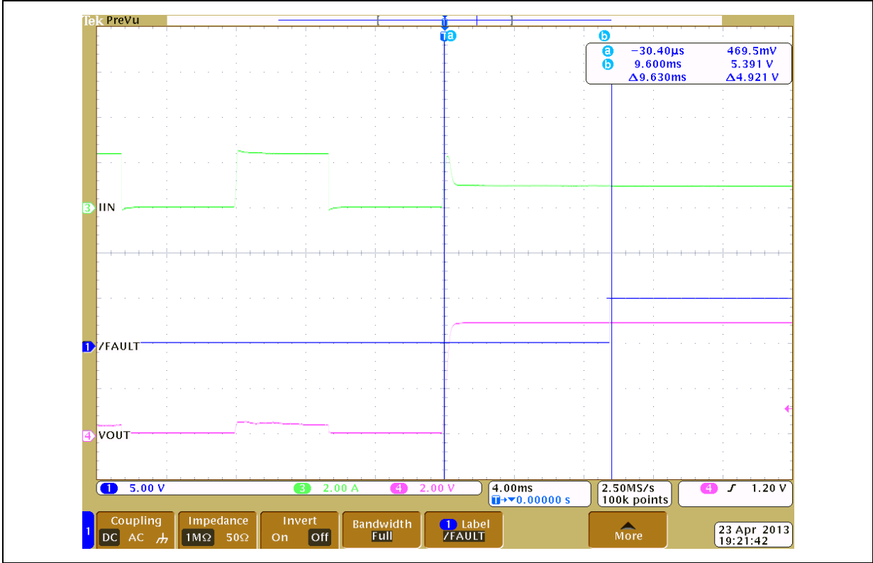
Figure 29. Short-circuit to full load recovery ( R_{ILIM} = 20\text{ k}\Omega , R_{LOAD} = 5\text{ }\Omega , C_{LOAD} = 150\text{ }\mu\text{F} )
