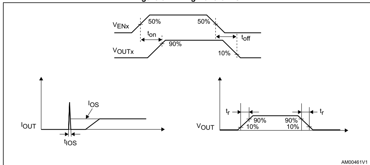
Figure 3. Timing waveforms
