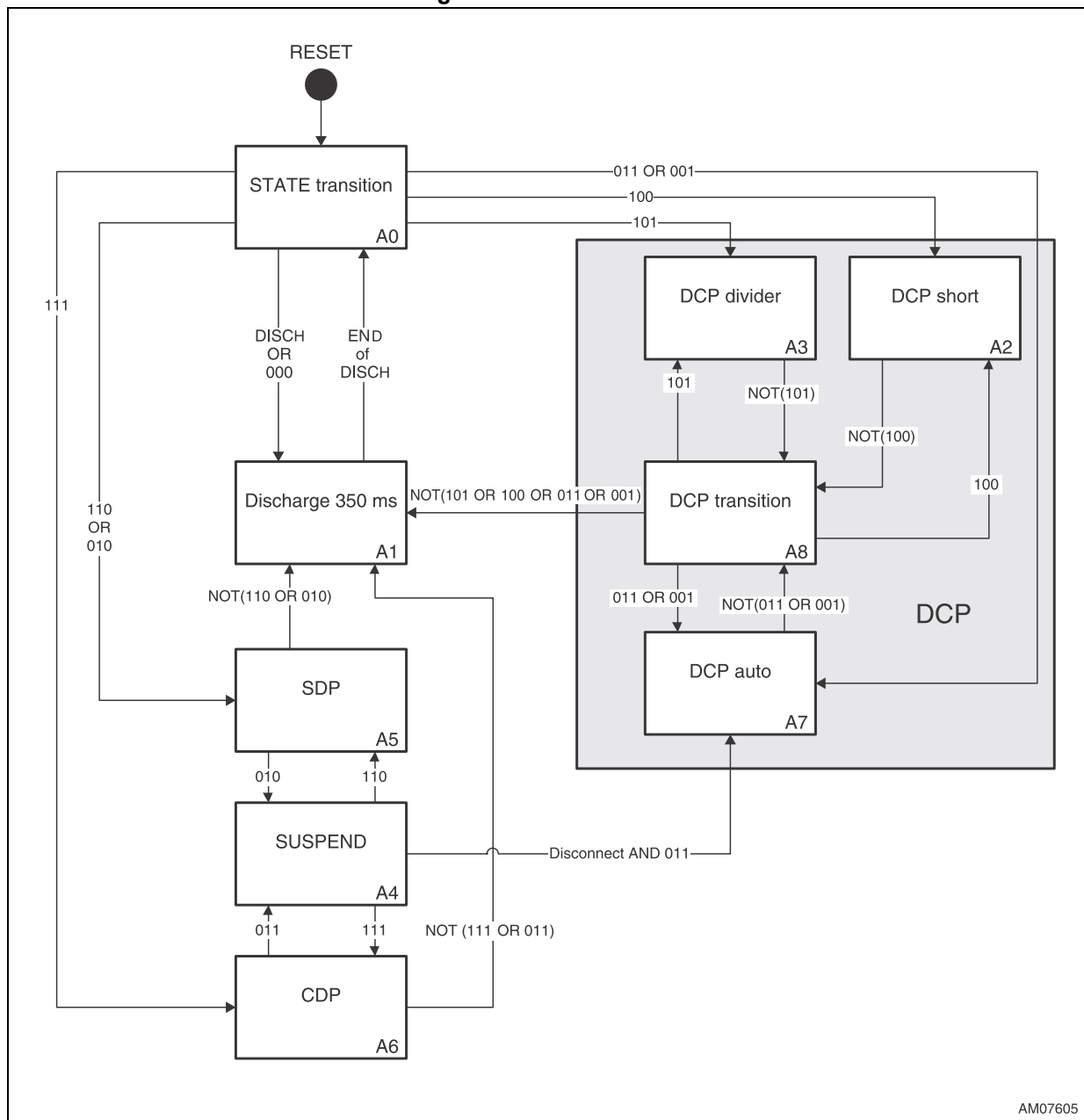
Figure 5. State machine
