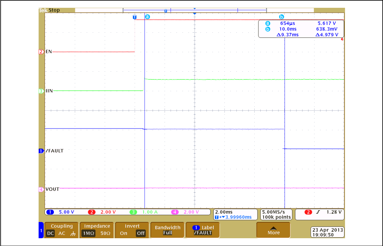
Figure 27. Device enabled into short-circuit ( R_{ILIM} = 80.6\text{ k}\Omega )
