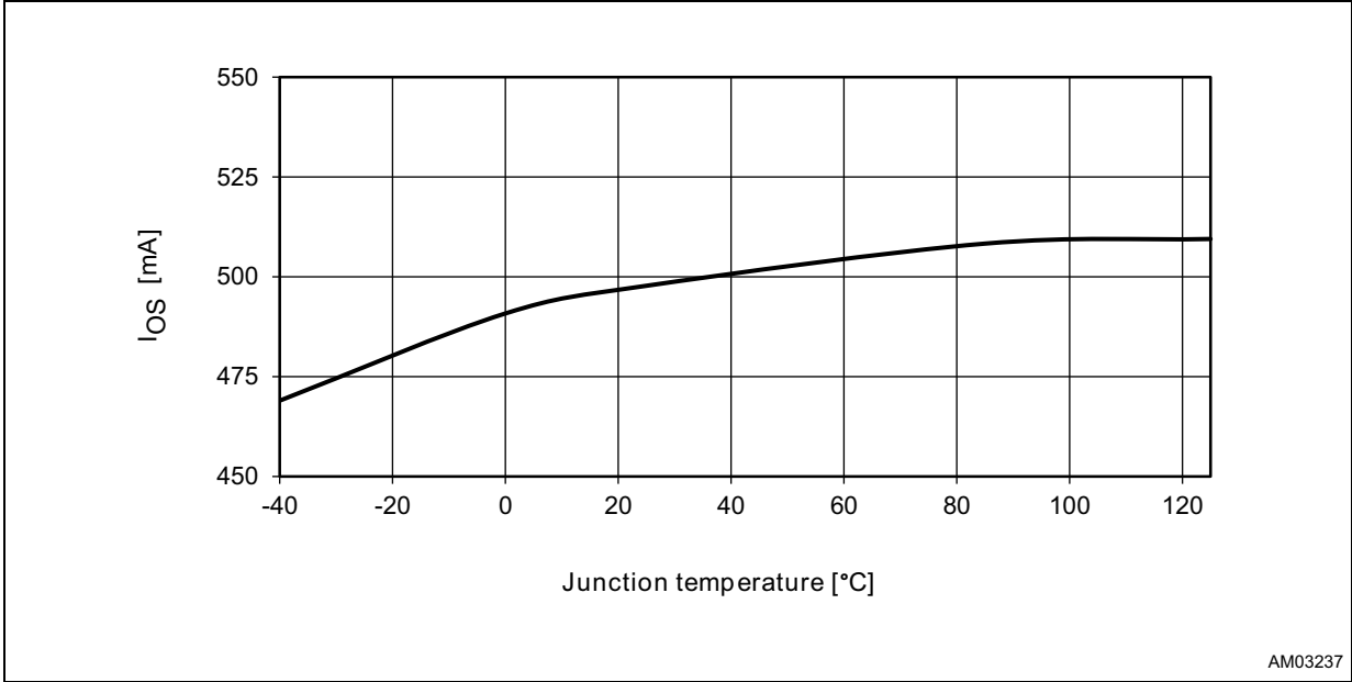
Figure 13. OUT short-circuit current limit vs. temperature ( R_{ILIM} = 96\text{ k}\Omega )
