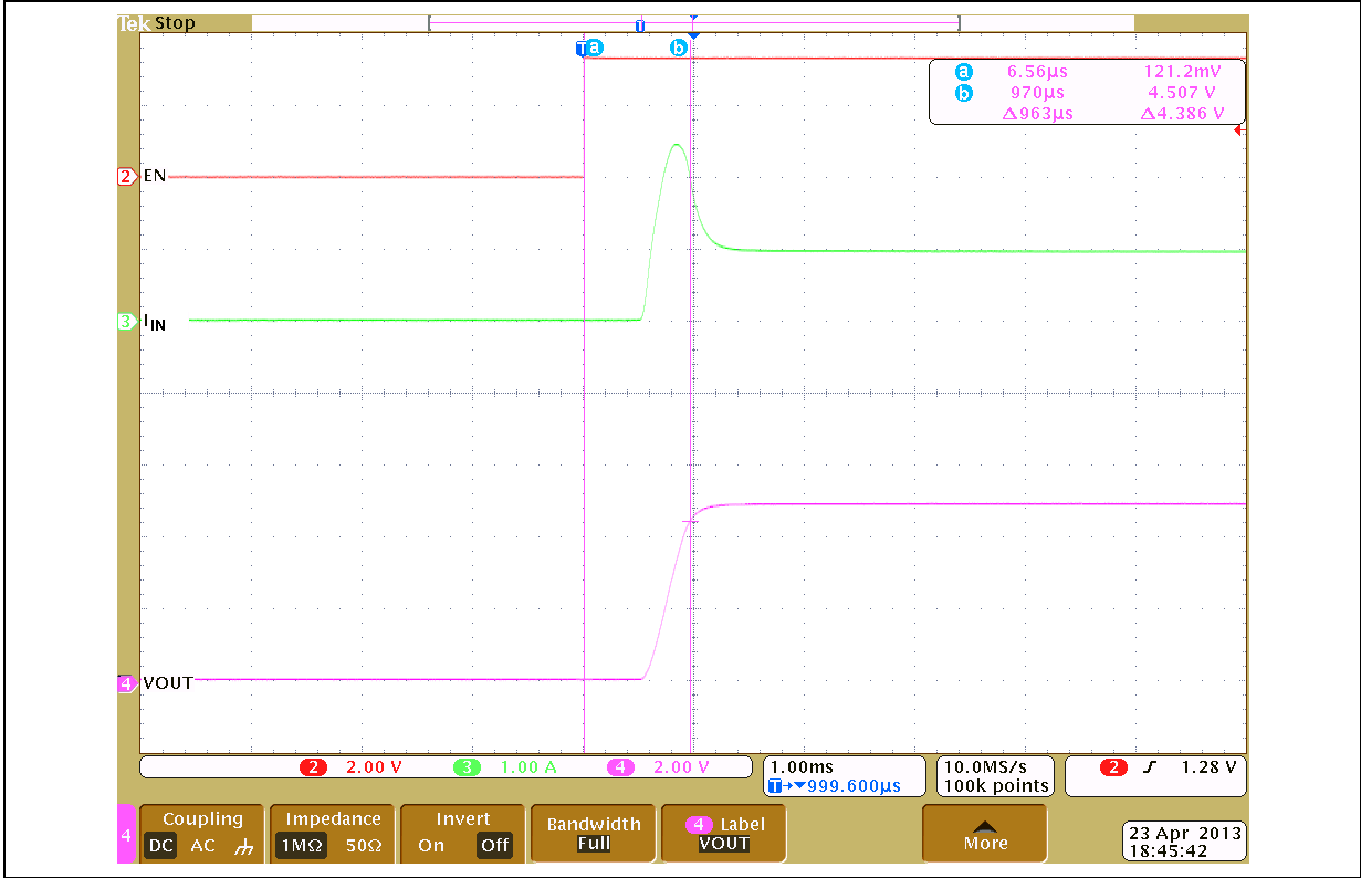
Figure 25. Turn-on response ( R_{ILIM} = 20\text{ k}\Omega , R_{LOAD} = 5\text{ }\Omega , C_{LOAD} = 150\text{ }\mu\text{F} )
